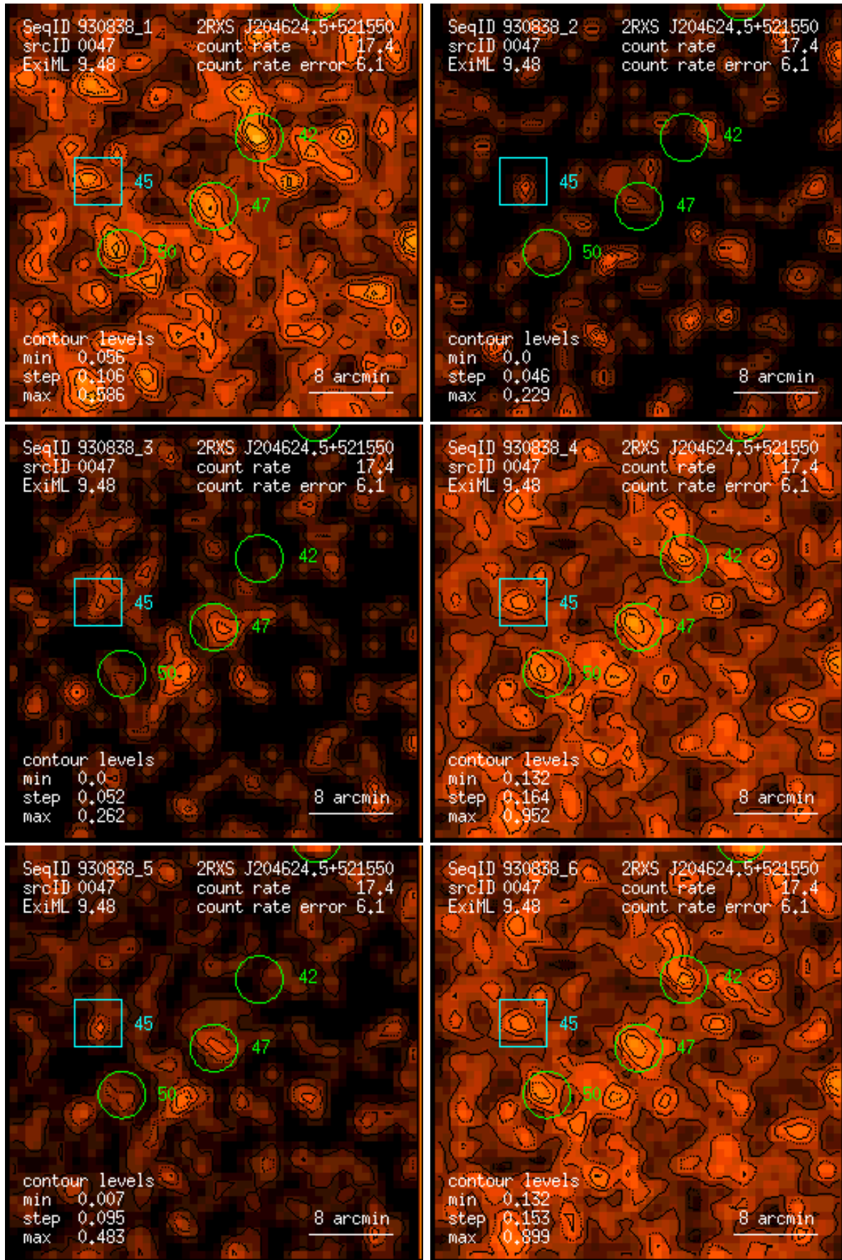
Figure 47: RASS 930838: detection 0047: band rate images, Gaussian filter: (1) PSPC channels 11 – 41, (2) 52 – 90, (3) 91 – 201, (4) 11 – 235, (5) 52 – 201, (6) 11 – 201. Broad band rates in counts/ks. Band rate contour levels in counts/ks/arcmin 2 .
