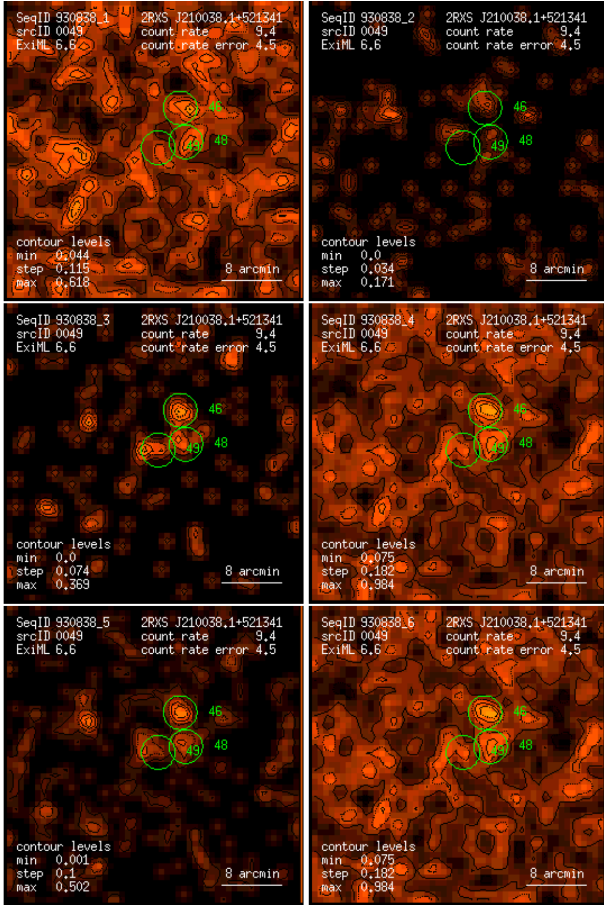
Figure 49: RASS 930838: detection 0049: band rate images, Gaussian filter: (1) PSPC channels 11 – 41, (2) 52 – 90, (3) 91 – 201, (4) 11 – 235, (5) 52 – 201, (6) 11 – 201. Broad band rates in counts/ks. Band rate contour levels in counts/ks/arcmin 2 .
