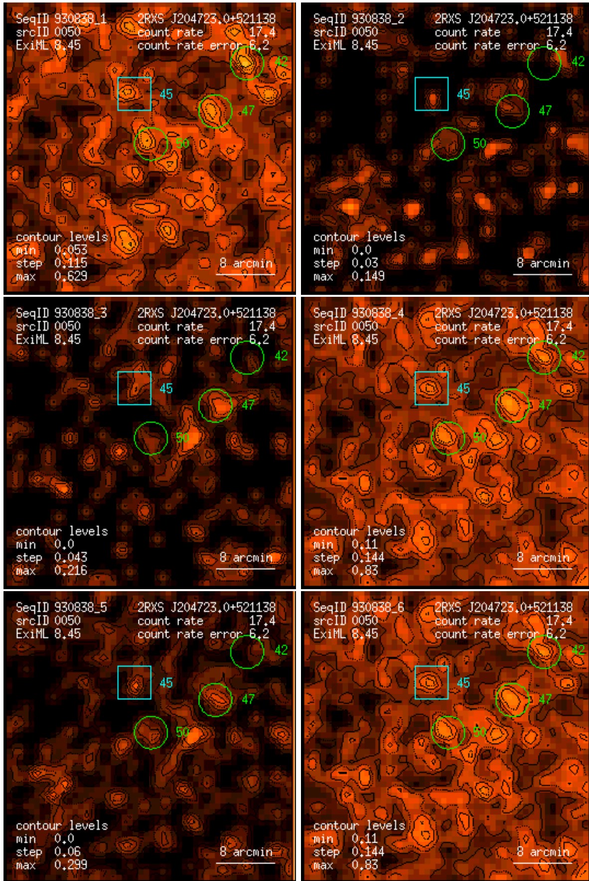
Figure 50: RASS 930838: detection 0050: band rate images, Gaussian filter: (1) PSPC channels 11 – 41, (2) 52 – 90, (3) 91 – 201, (4) 11 – 235, (5) 52 – 201, (6) 11 – 201. Broad band rates in counts/ks. Band rate contour levels in counts/ks/arcmin 2 .
