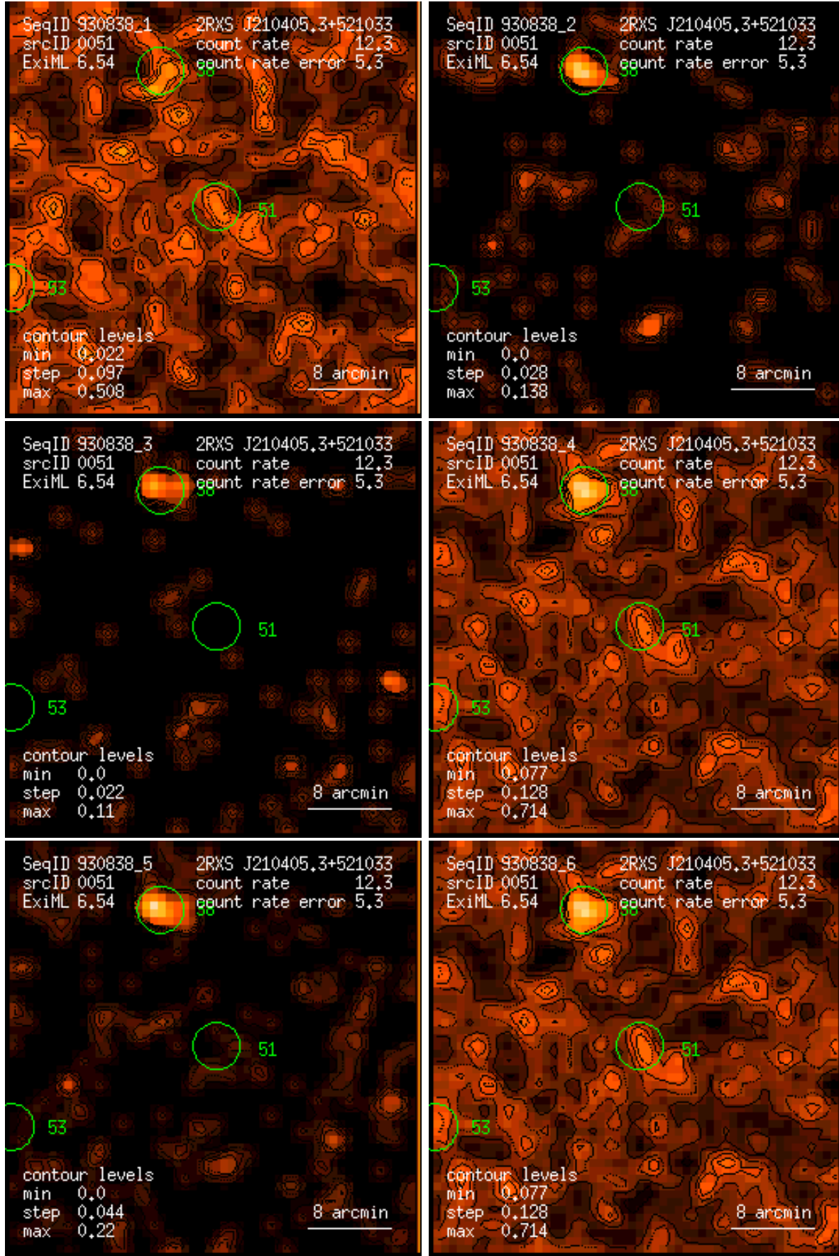
Figure 51: RASS 930838: detection 0051: band rate images, Gaussian filter: (1) PSPC channels 11 – 41, (2) 52 – 90, (3) 91 – 201, (4) 11 – 235, (5) 52 – 201, (6) 11 – 201. Broad band rates in counts/ks. Band rate contour levels in counts/ks/arcmin 2 .
