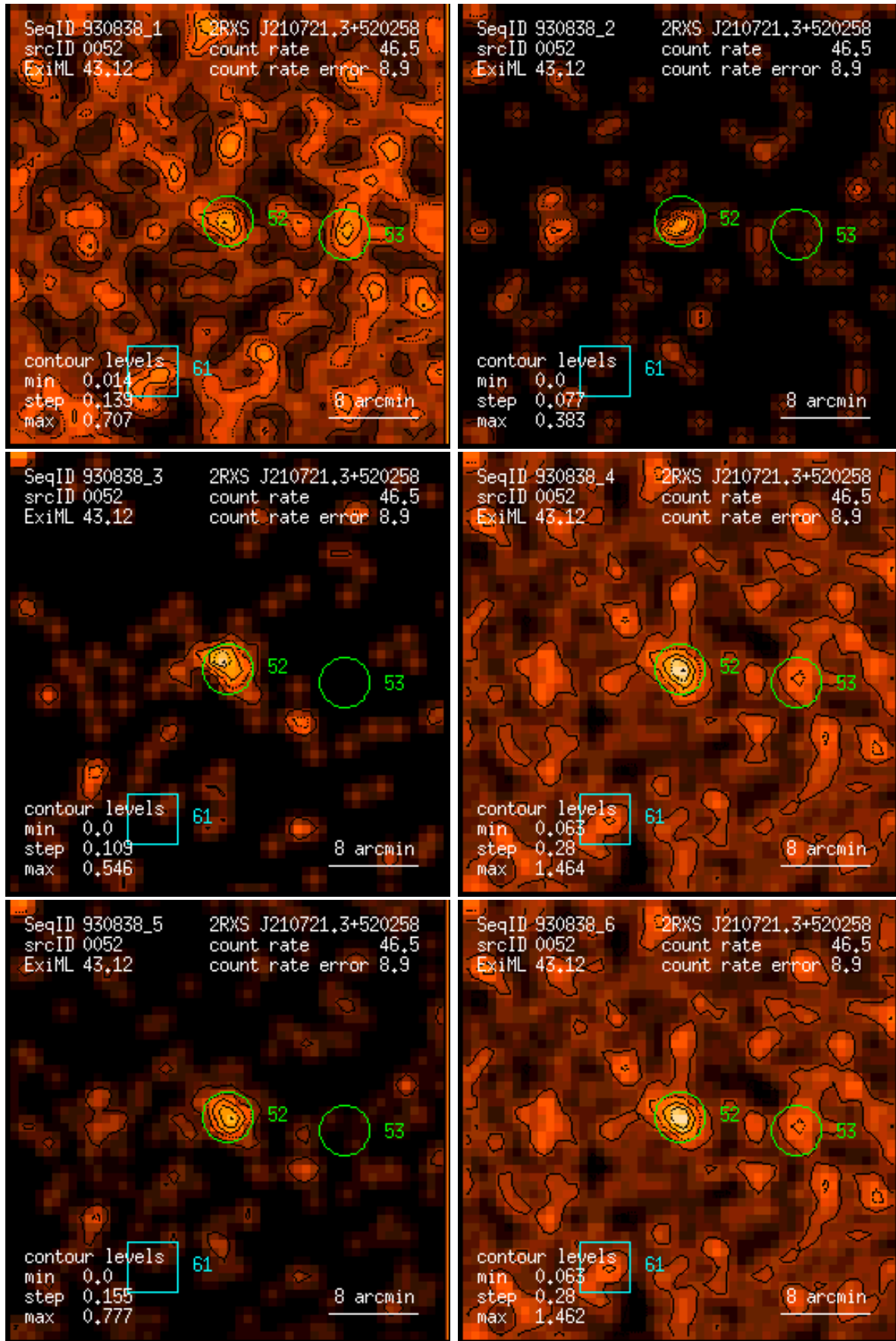
Figure 52: RASS 930838: detection 0052: band rate images, Gaussian filter: (1) PSPC channels 11 – 41, (2) 52 – 90, (3) 91 – 201, (4) 11 – 235, (5) 52 – 201, (6) 11 – 201. Broad band rates in counts/ks. Band rate contour levels in counts/ks/arcmin 2 .
