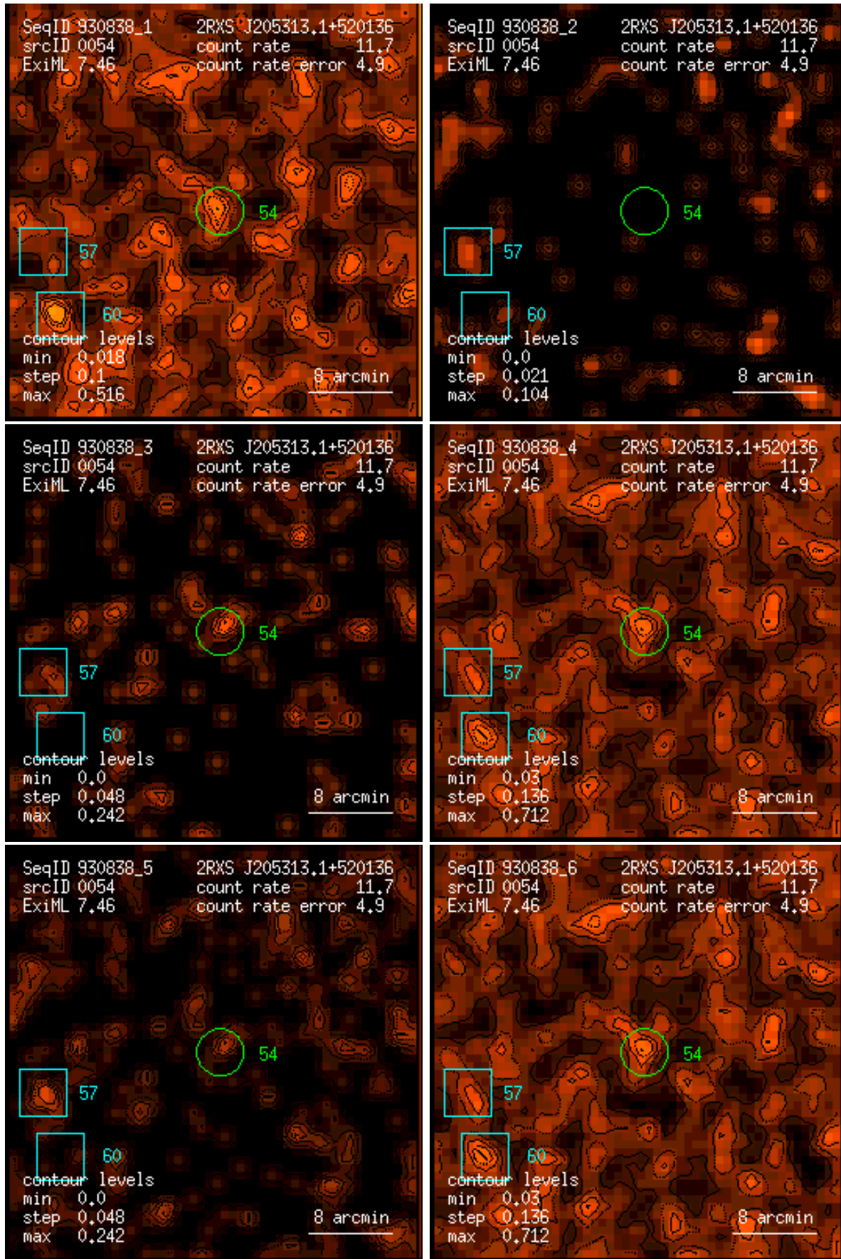
Figure 54: RASS 930838: detection 0054: band rate images, Gaussian filter: (1) PSPC channels 11 – 41, (2) 52 – 90, (3) 91 – 201, (4) 11 – 235, (5) 52 – 201, (6) 11 – 201. Broad band rates in counts/ks. Band rate contour levels in counts/ks/arcmin 2 .
