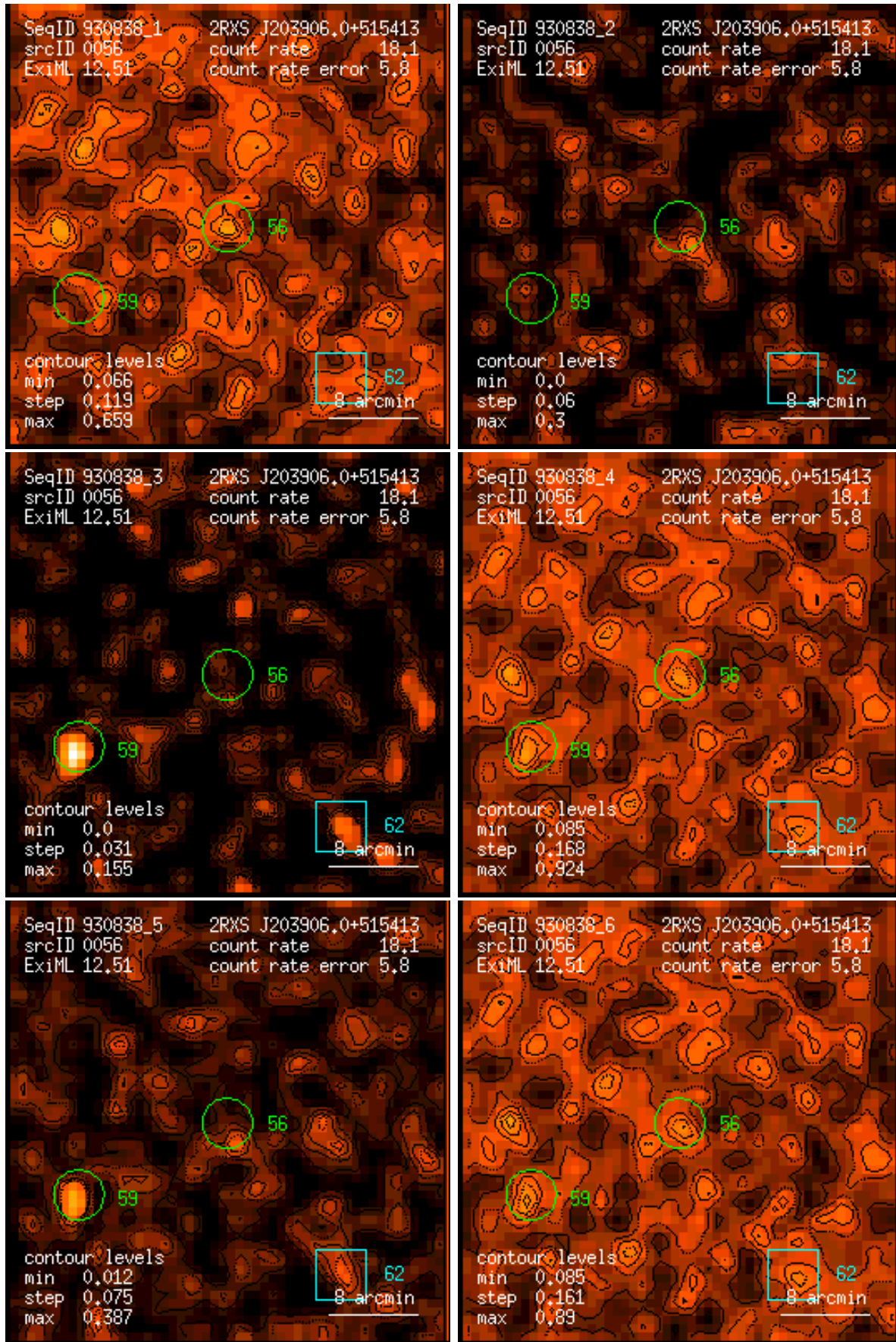
Figure 56: RASS 930838: detection 0056: band rate images, Gaussian filter: (1) PSPC channels 11 – 41, (2) 52 – 90, (3) 91 – 201, (4) 11 – 235, (5) 52 – 201, (6) 11 – 201. Broad band rates in counts/ks. Band rate contour levels in counts/ks/arcmin 2 .
