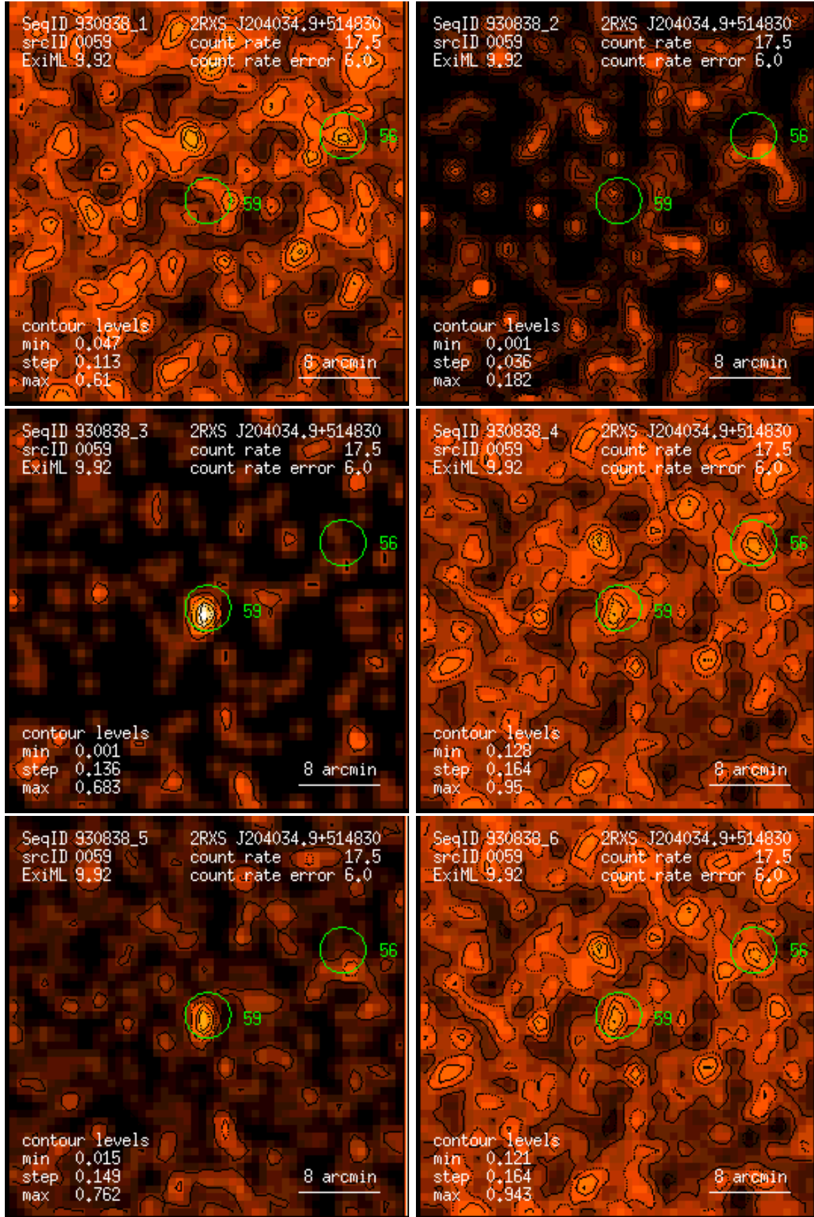
Figure 59: RASS 930838: detection 0059: band rate images, Gaussian filter: (1) PSPC channels 11 – 41, (2) 52 – 90, (3) 91 – 201, (4) 11 – 235, (5) 52 – 201, (6) 11 – 201. Broad band rates in counts/ks. Band rate contour levels in counts/ks/arcmin 2 .
