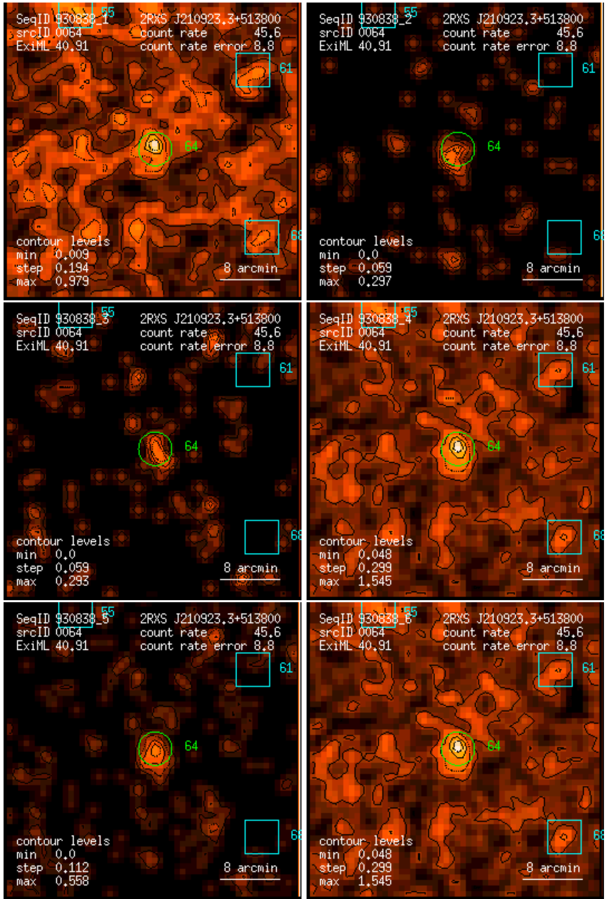
Figure 64: RASS 930838: detection 0064: band rate images, Gaussian filter: (1) PSPC channels 11 – 41, (2) 52 – 90, (3) 91 – 201, (4) 11 – 235, (5) 52 – 201, (6) 11 – 201. Broad band rates in counts/ks. Band rate contour levels in counts/ks/arcmin 2 .
