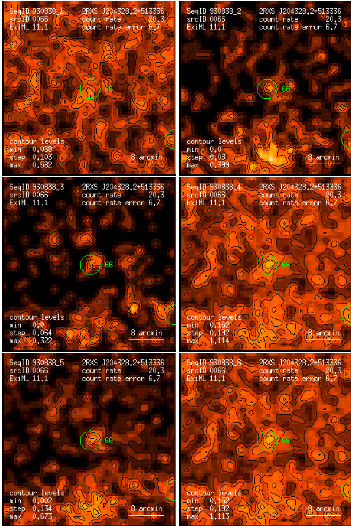
Figure 66: RASS 930838: detection 0066: band rate images, Gaussian filter: (1) PSPC channels 11 – 41, (2) 52 – 90, (3) 91 – 201, (4) 11 – 235, (5) 52 – 201, (6) 11 – 201. Broad band rates in counts/ks. Band rate contour levels in counts/ks/arcmin 2 .
