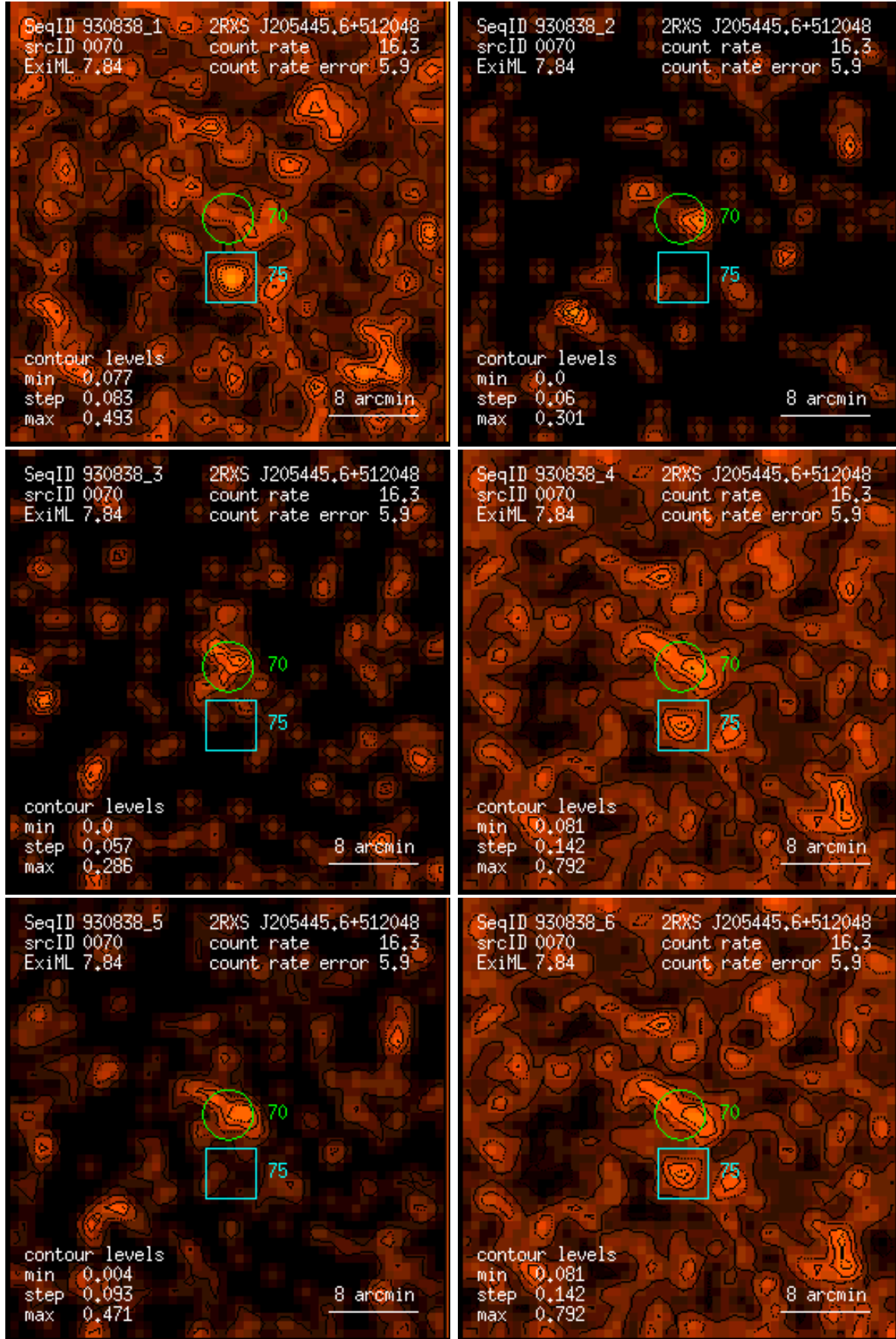
Figure 70: RASS 930838: detection 0070: band rate images, Gaussian filter: (1) PSPC channels 11 – 41, (2) 52 – 90, (3) 91 – 201, (4) 11 – 235, (5) 52 – 201, (6) 11 – 201. Broad band rates in counts/ks. Band rate contour levels in counts/ks/arcmin 2 .
