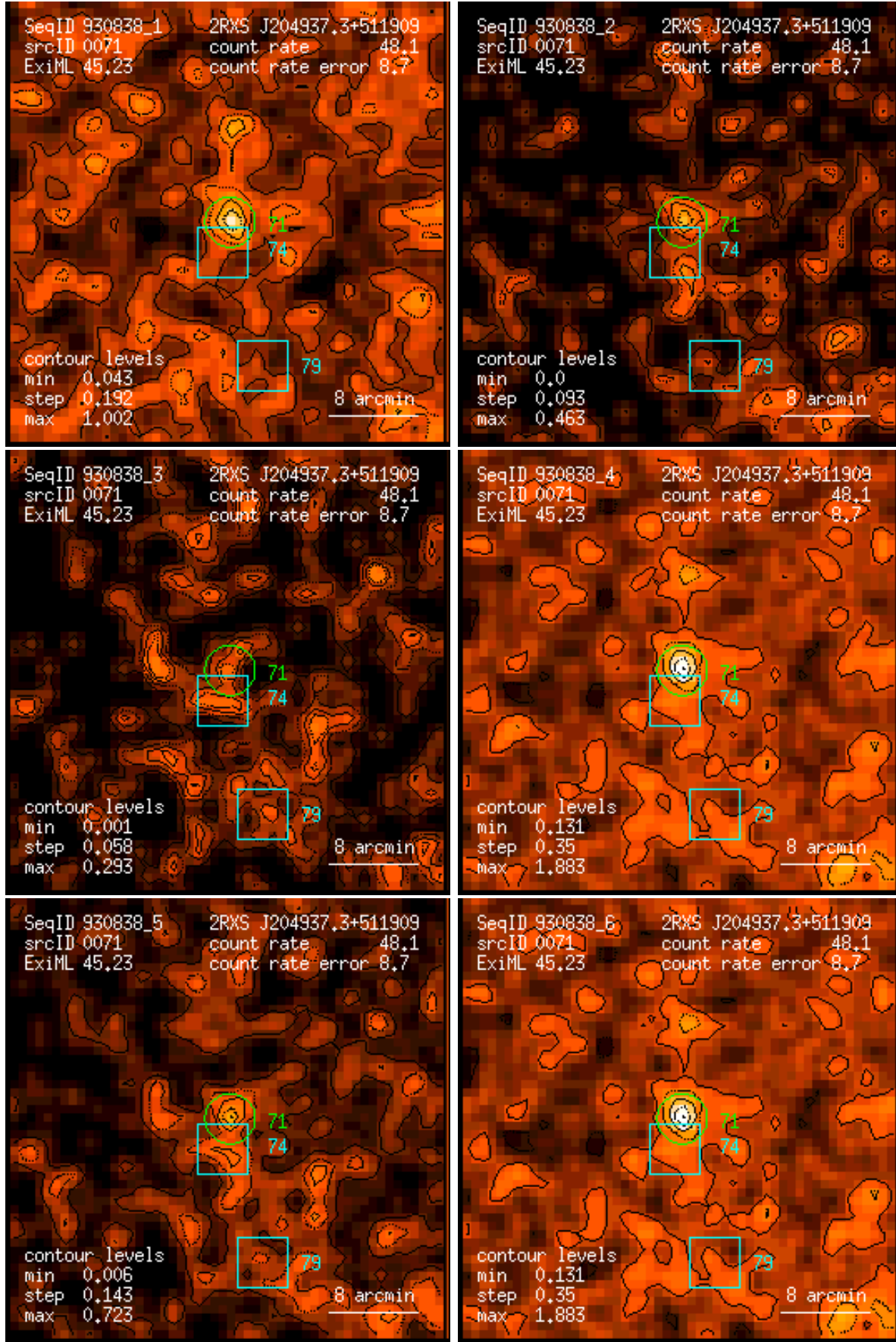
Figure 71: RASS 930838: detection 0071: band rate images, Gaussian filter: (1) PSPC channels 11 – 41, (2) 52 – 90, (3) 91 – 201, (4) 11 – 235, (5) 52 – 201, (6) 11 – 201. Broad band rates in counts/ks. Band rate contour levels in counts/ks/arcmin 2 .
