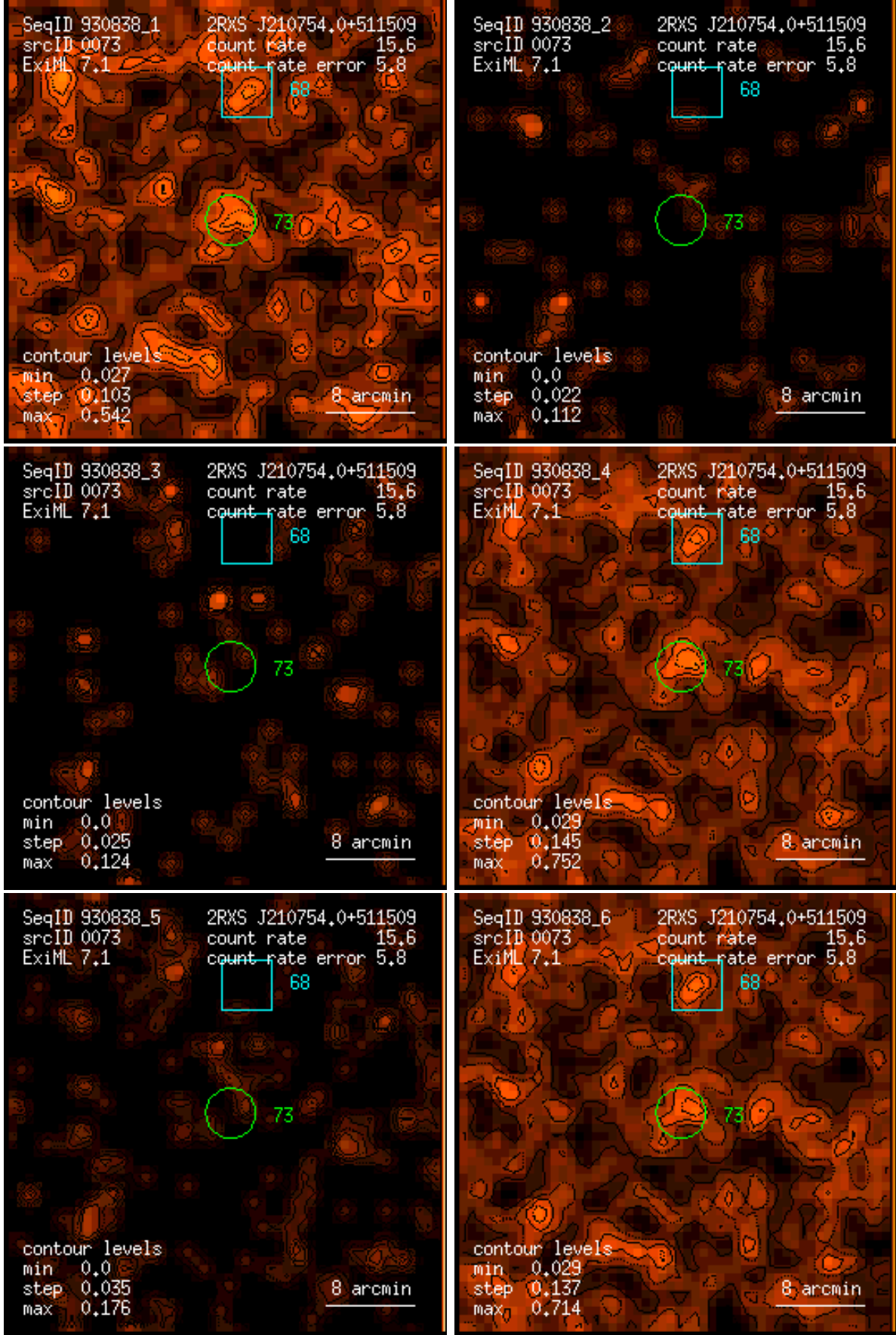
Figure 73: RASS 930838: detection 0073: band rate images, Gaussian filter: (1) PSPC channels 11 – 41, (2) 52 – 90, (3) 91 – 201, (4) 11 – 235, (5) 52 – 201, (6) 11 – 201. Broad band rates in counts/ks. Band rate contour levels in counts/ks/arcmin 2 .
