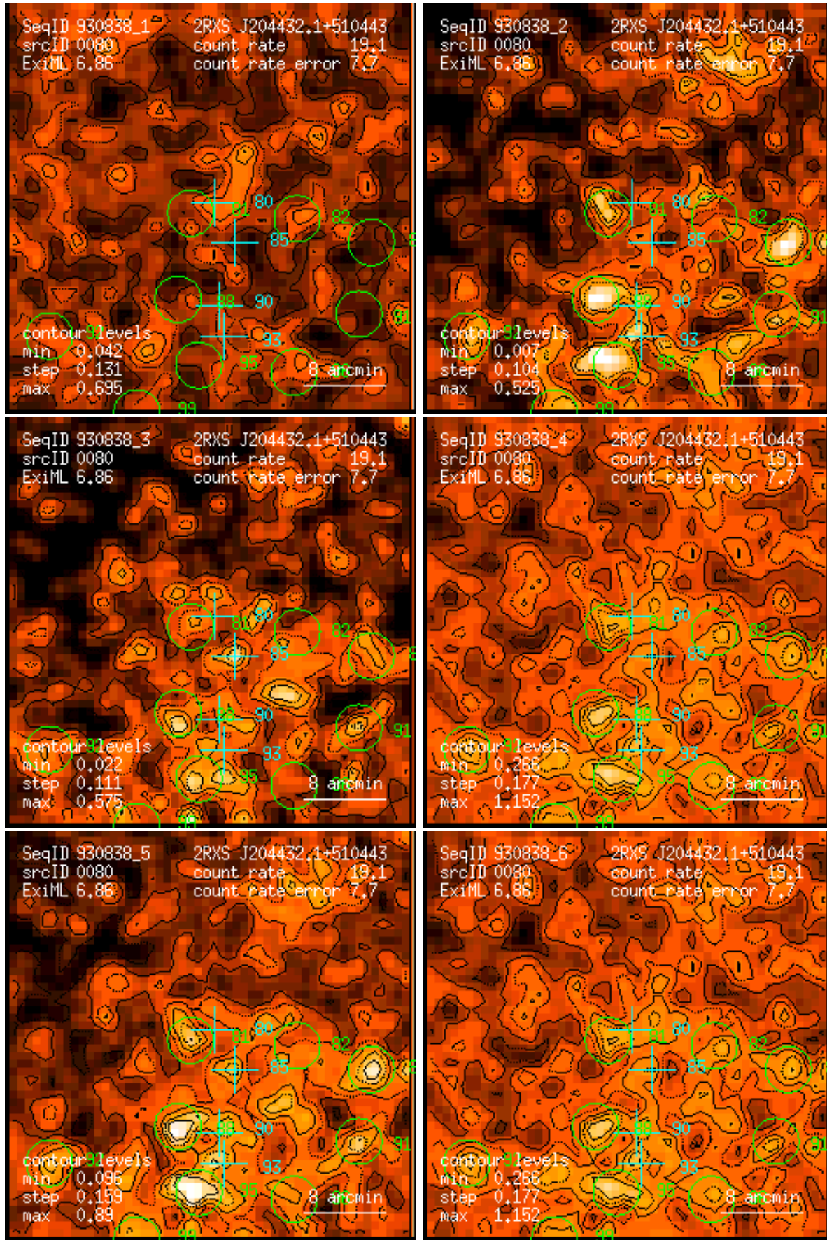
Figure 80: RASS 930838: detection 0080: band rate images, Gaussian filter: (1) PSPC channels 11 – 41, (2) 52 – 90, (3) 91 – 201, (4) 11 – 235, (5) 52 – 201, (6) 11 – 201. Broad band rates in counts/ks. Band rate contour levels in counts/ks/arcmin 2 .
