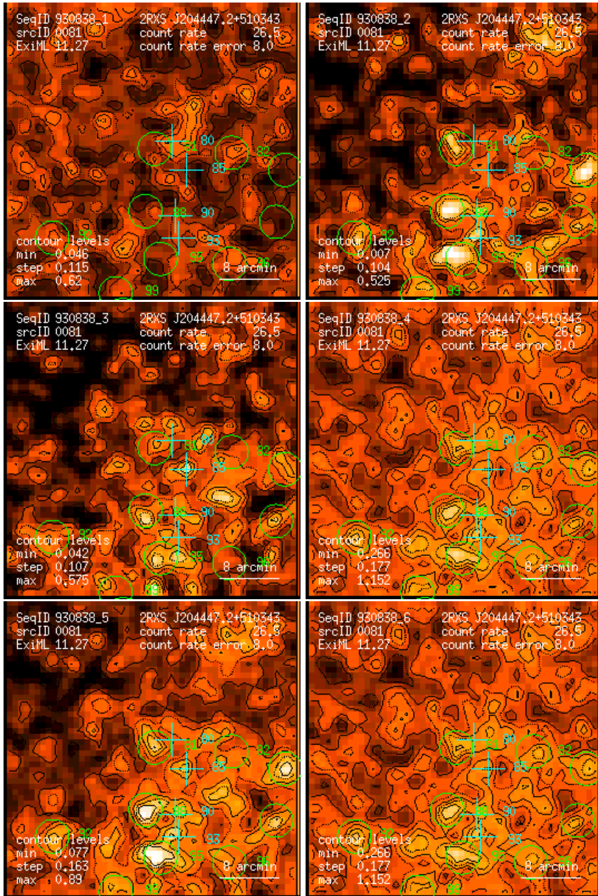
Figure 81: RASS 930838: detection 0081: band rate images, Gaussian filter: (1) PSPC channels 11 – 41, (2) 52 – 90, (3) 91 – 201, (4) 11 – 235, (5) 52 – 201, (6) 11 – 201. Broad band rates in counts/ks. Band rate contour levels in counts/ks/arcmin 2 .
