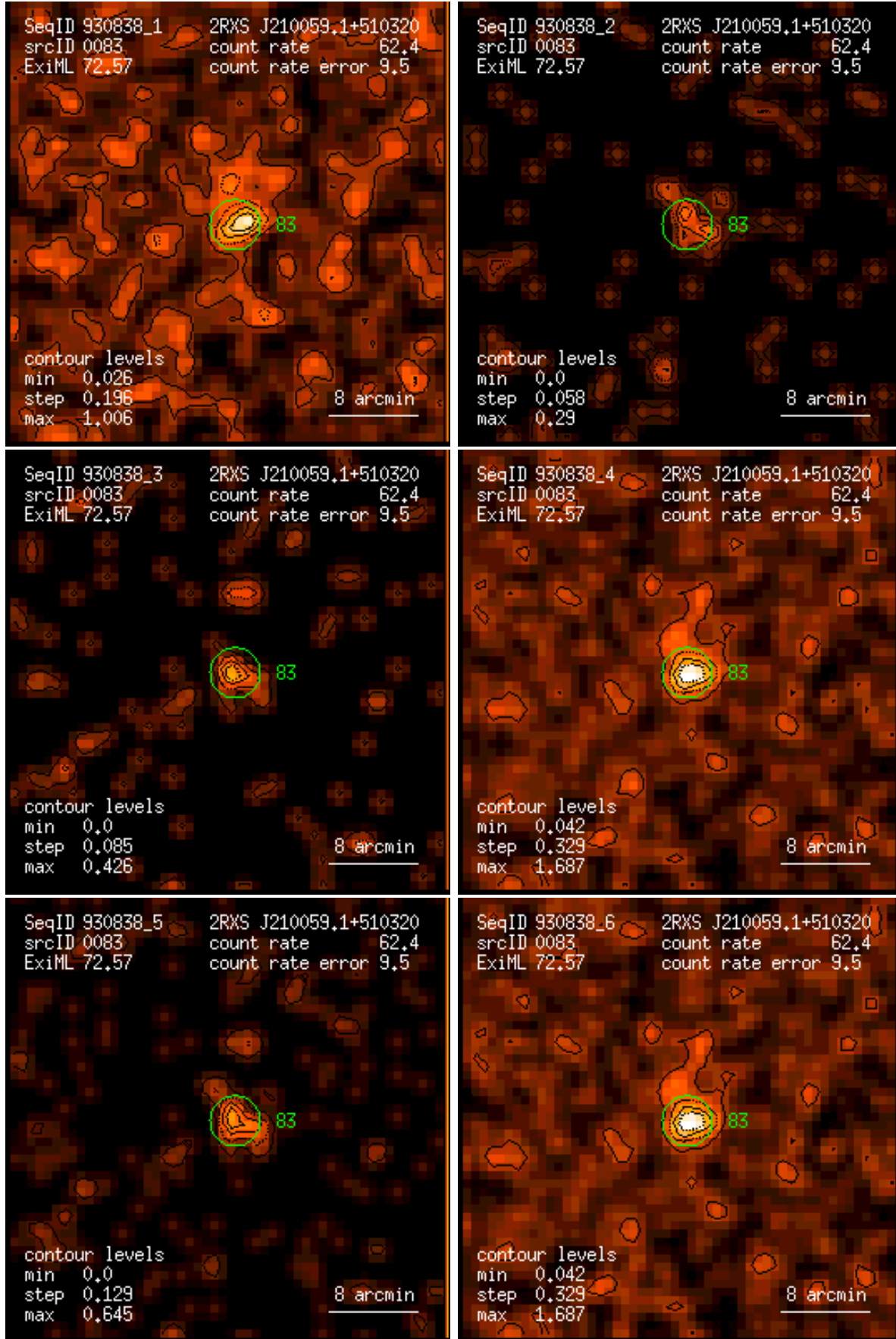
Figure 83: RASS 930838: detection 0083: band rate images, Gaussian filter: (1) PSPC channels 11 – 41, (2) 52 – 90, (3) 91 – 201, (4) 11 – 235, (5) 52 – 201, (6) 11 – 201. Broad band rates in counts/ks. Band rate contour levels in counts/ks/arcmin 2 .
