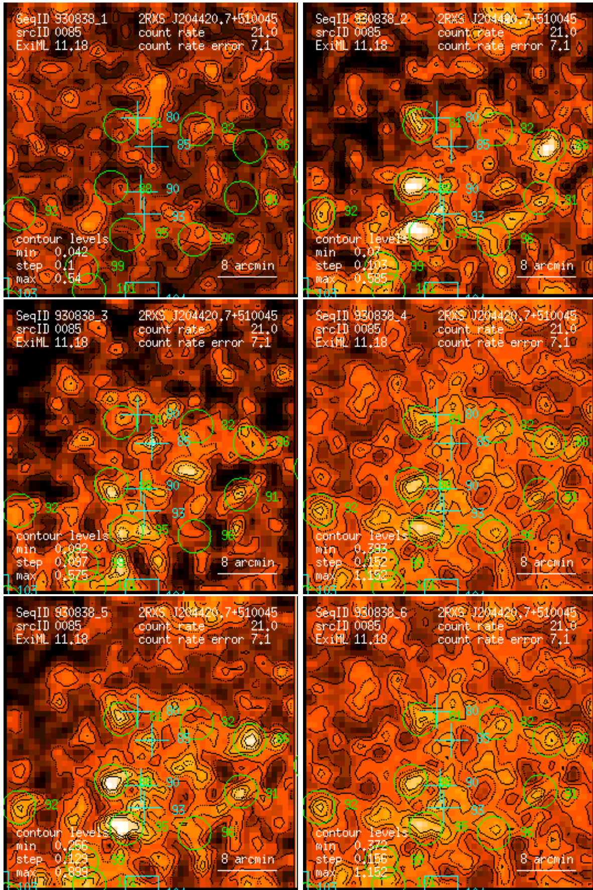
Figure 85: RASS 930838: detection 0085: band rate images, Gaussian filter: (1) PSPC channels 11 – 41, (2) 52 – 90, (3) 91 – 201, (4) 11 – 235, (5) 52 – 201, (6) 11 – 201. Broad band rates in counts/ks. Band rate contour levels in counts/ks/arcmin 2 .
