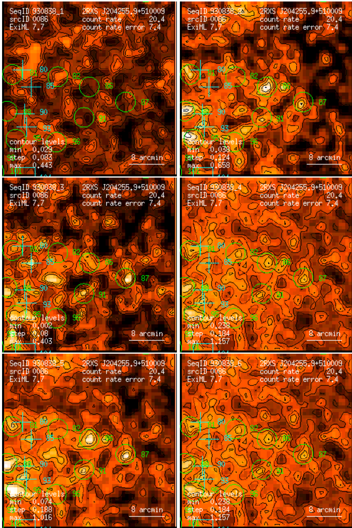
Figure 86: RASS 930838: detection 0086: band rate images, Gaussian filter: (1) PSPC channels 11 – 41, (2) 52 – 90, (3) 91 – 201, (4) 11 – 235, (5) 52 – 201, (6) 11 – 201. Broad band rates in counts/ks. Band rate contour levels in counts/ks/arcmin 2 .
