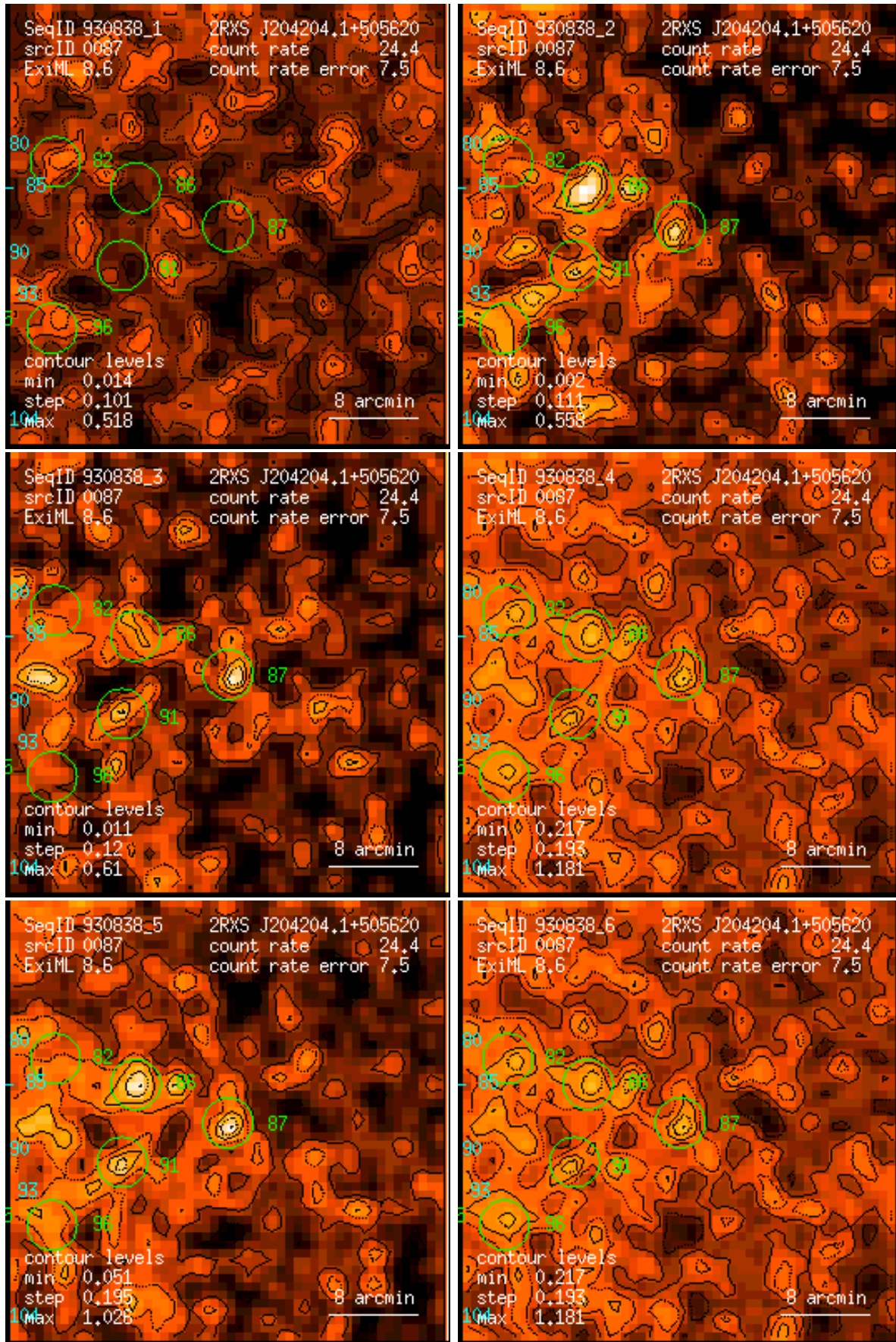
Figure 87: RASS 930838: detection 0087: band rate images, Gaussian filter: (1) PSPC channels 11 – 41, (2) 52 – 90, (3) 91 – 201, (4) 11 – 235, (5) 52 – 201, (6) 11 – 201. Broad band rates in counts/ks. Band rate contour levels in counts/ks/arcmin 2 .
