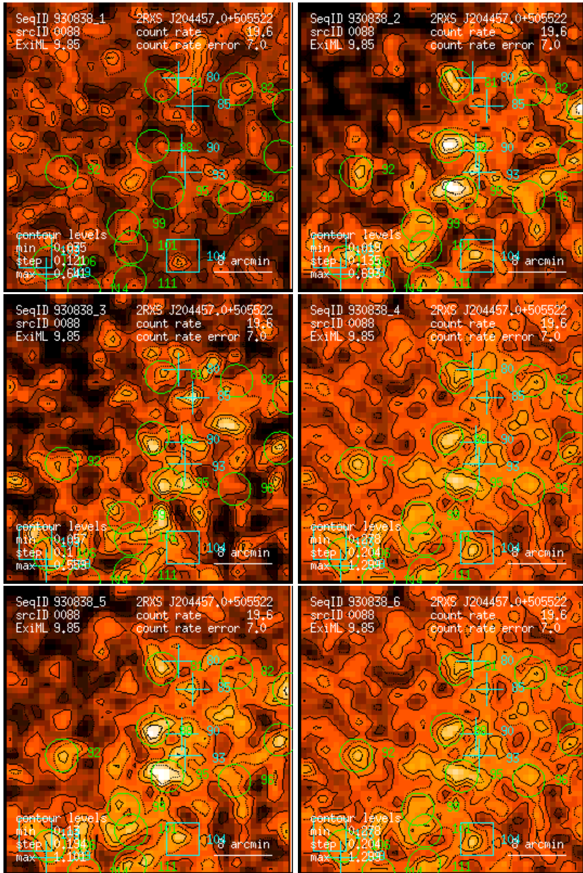
Figure 88: RASS 930838: detection 0088: band rate images, Gaussian filter: (1) PSPC channels 11 – 41, (2) 52 – 90, (3) 91 – 201, (4) 11 – 235, (5) 52 – 201, (6) 11 – 201. Broad band rates in counts/ks. Band rate contour levels in counts/ks/arcmin 2 .
