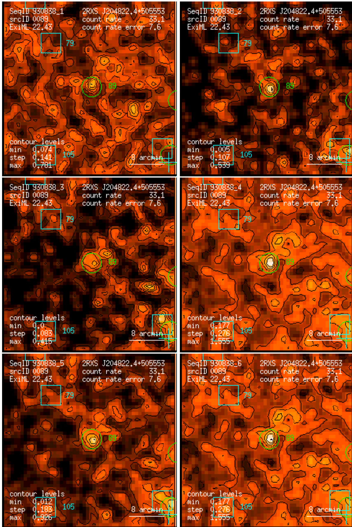
Figure 89: RASS 930838: detection 0089: band rate images, Gaussian filter: (1) PSPC channels 11 – 41, (2) 52 – 90, (3) 91 – 201, (4) 11 – 235, (5) 52 – 201, (6) 11 – 201. Broad band rates in counts/ks. Band rate contour levels in counts/ks/arcmin 2 .
