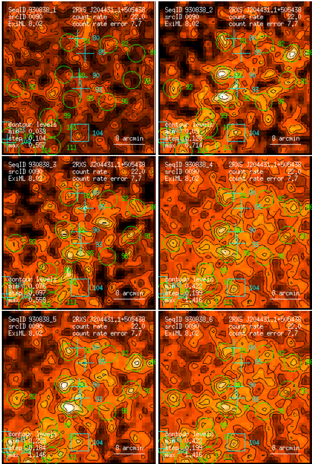
Figure 90: RASS 930838: detection 0090: band rate images, Gaussian filter: (1) PSPC channels 11 – 41, (2) 52 – 90, (3) 91 – 201, (4) 11 – 235, (5) 52 – 201, (6) 11 – 201. Broad band rates in counts/ks. Band rate contour levels in counts/ks/arcmin 2 .
