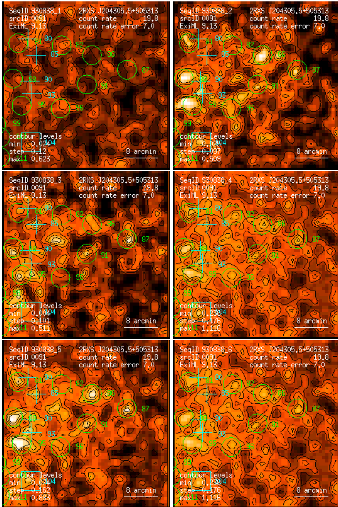
Figure 91: RASS 930838: detection 0091: band rate images, Gaussian filter: (1) PSPC channels 11 – 41, (2) 52 – 90, (3) 91 – 201, (4) 11 – 235, (5) 52 – 201, (6) 11 – 201. Broad band rates in counts/ks. Band rate contour levels in counts/ks/arcmin 2 .
