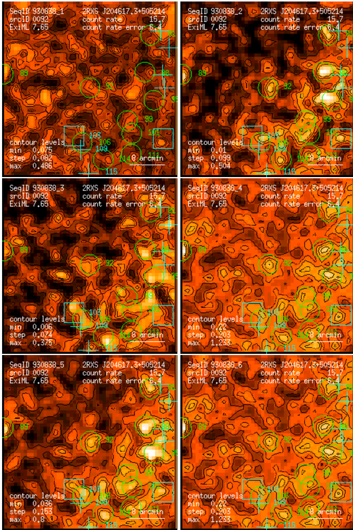
Figure 92: RASS 930838: detection 0092: band rate images, Gaussian filter: (1) PSPC channels 11 – 41, (2) 52 – 90, (3) 91 – 201, (4) 11 – 235, (5) 52 – 201, (6) 11 – 201. Broad band rates in counts/ks. Band rate contour levels in counts/ks/arcmin 2 .
