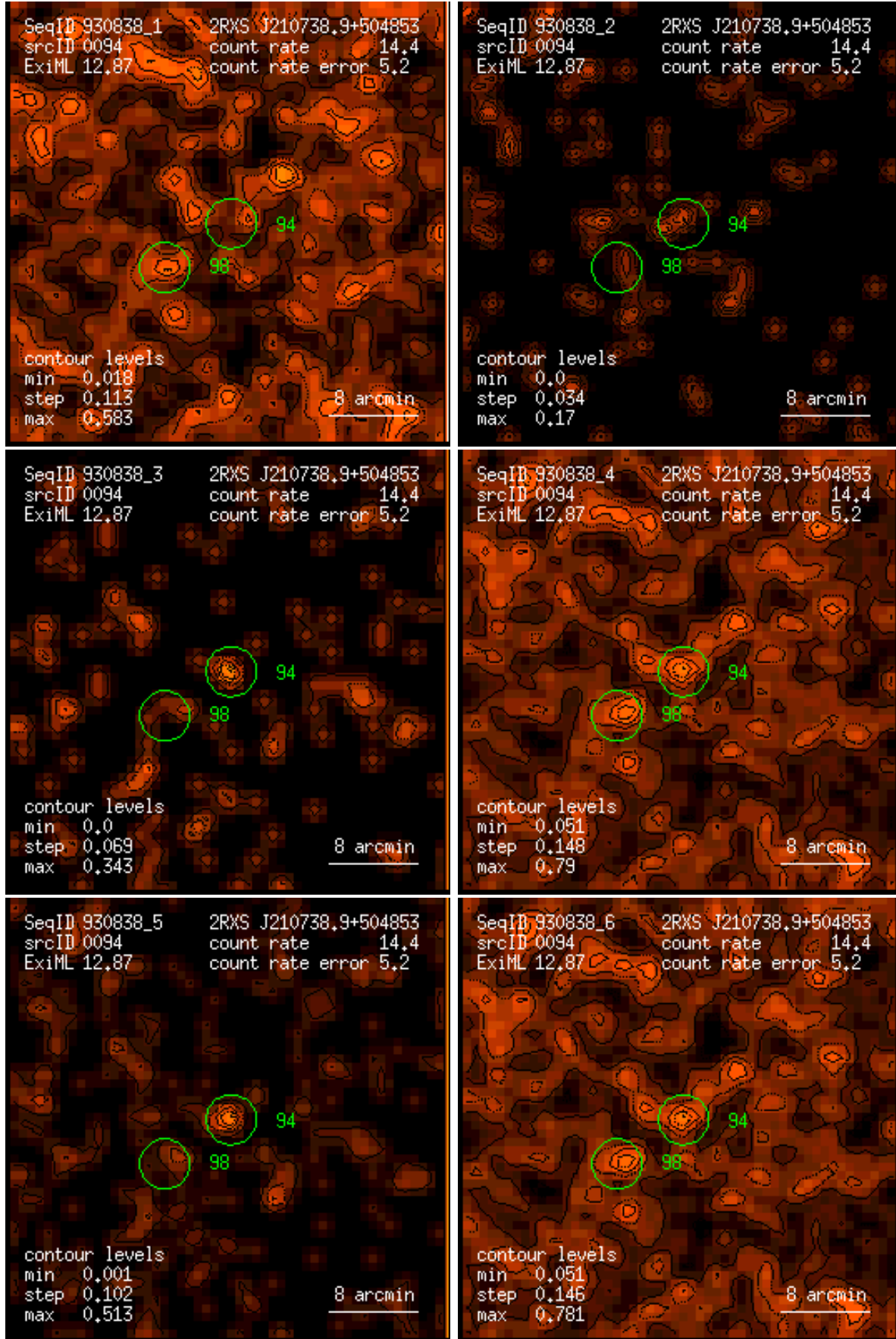
Figure 94: RASS 930838: detection 0094: band rate images, Gaussian filter: (1) PSPC channels 11 – 41, (2) 52 – 90, (3) 91 – 201, (4) 11 – 235, (5) 52 – 201, (6) 11 – 201. Broad band rates in counts/ks. Band rate contour levels in counts/ks/arcmin 2 .
