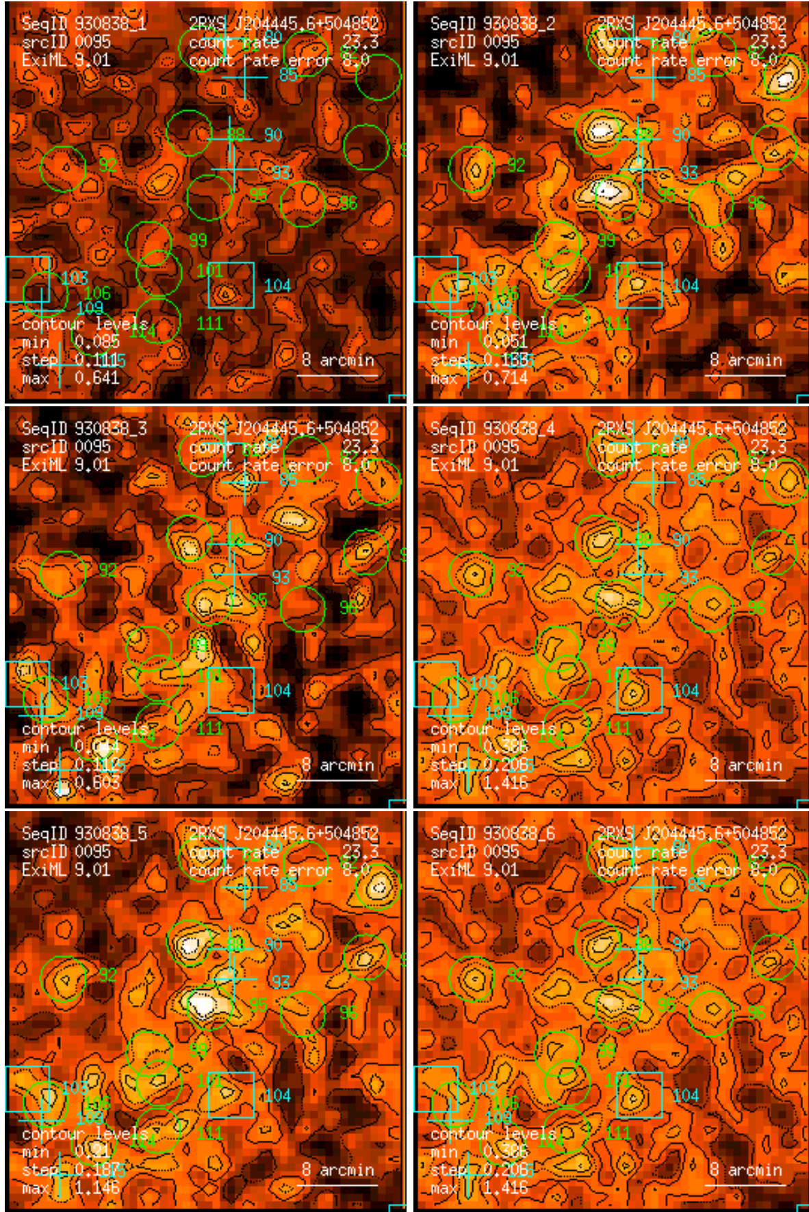
Figure 95: RASS 930838: detection 0095: band rate images, Gaussian filter: (1) PSPC channels 11 – 41, (2) 52 – 90, (3) 91 – 201, (4) 11 – 235, (5) 52 – 201, (6) 11 – 201. Broad band rates in counts/ks. Band rate contour levels in counts/ks/arcmin 2 .
