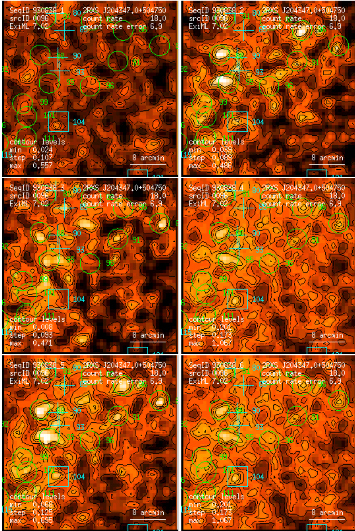
Figure 96: RASS 930838: detection 0096: band rate images, Gaussian filter: (1) PSPC channels 11 – 41, (2) 52 – 90, (3) 91 – 201, (4) 11 – 235, (5) 52 – 201, (6) 11 – 201. Broad band rates in counts/ks. Band rate contour levels in counts/ks/arcmin 2 .
