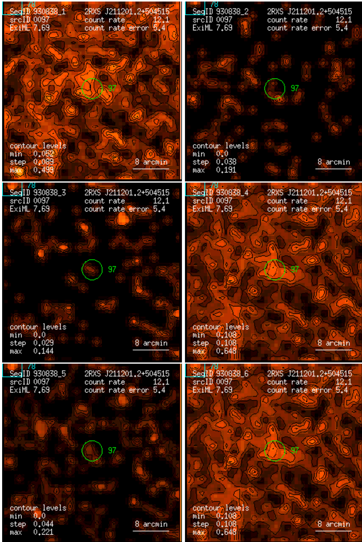
Figure 97: RASS 930838: detection 0097: band rate images, Gaussian filter: (1) PSPC channels 11 – 41, (2) 52 – 90, (3) 91 – 201, (4) 11 – 235, (5) 52 – 201, (6) 11 – 201. Broad band rates in counts/ks. Band rate contour levels in counts/ks/arcmin 2 .
