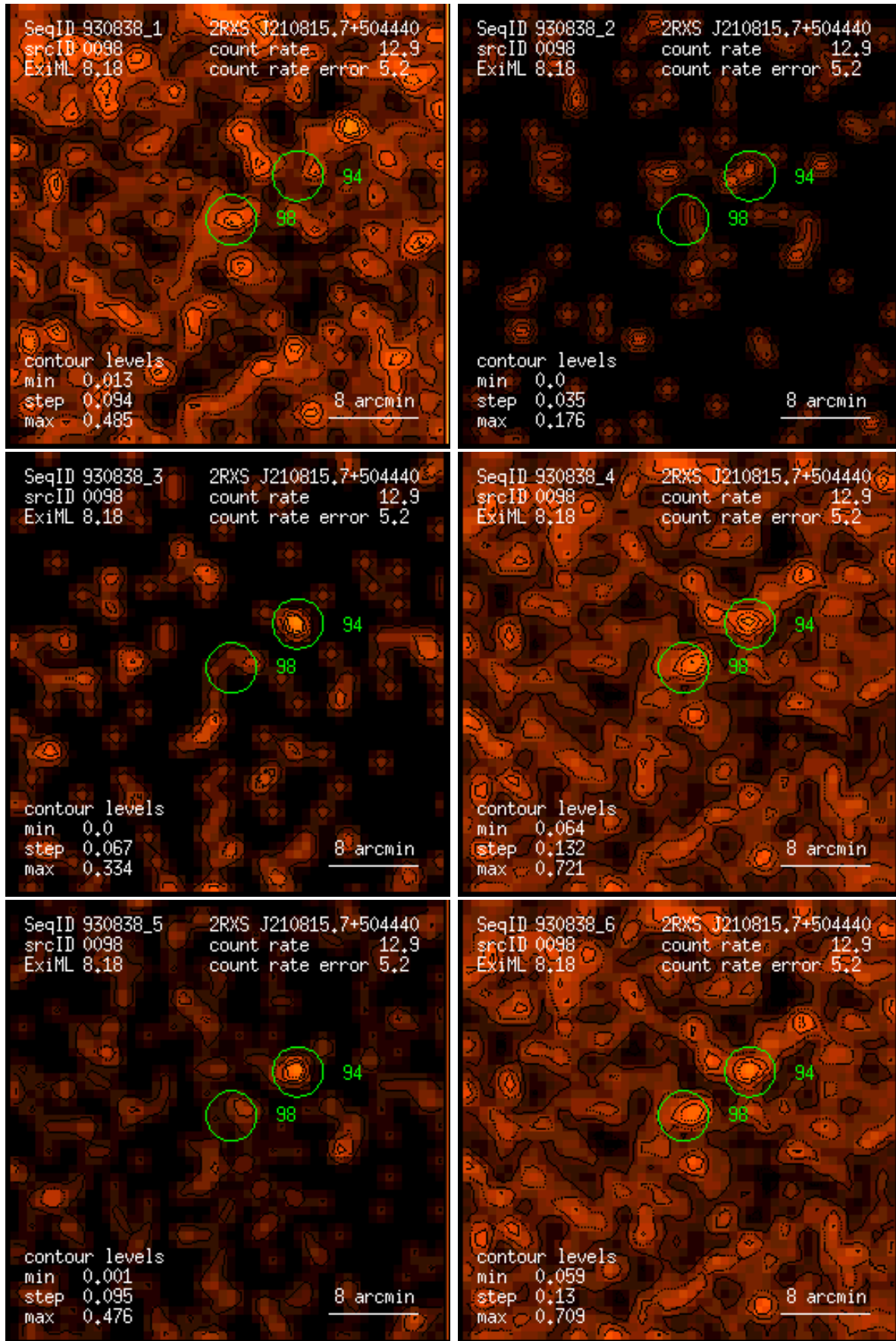
Figure 98: RASS 930838: detection 0098: band rate images, Gaussian filter: (1) PSPC channels 11 – 41, (2) 52 – 90, (3) 91 – 201, (4) 11 – 235, (5) 52 – 201, (6) 11 – 201. Broad band rates in counts/ks. Band rate contour levels in counts/ks/arcmin 2 .
