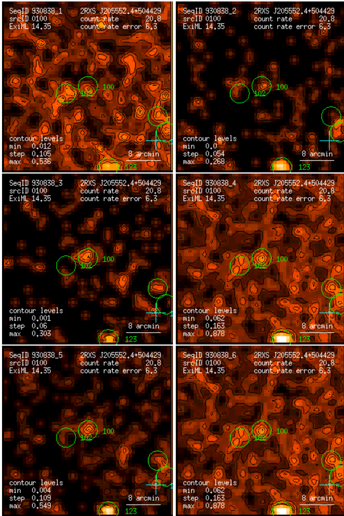
Figure 100: RASS 930838: detection 0100: band rate images, Gaussian filter: (1) PSPC channels 11 – 41, (2) 52 – 90, (3) 91 – 201, (4) 11 – 235, (5) 52 – 201, (6) 11 – 201. Broad band rates in counts/ks. Band rate contour levels in counts/ks/arcmin 2 .
