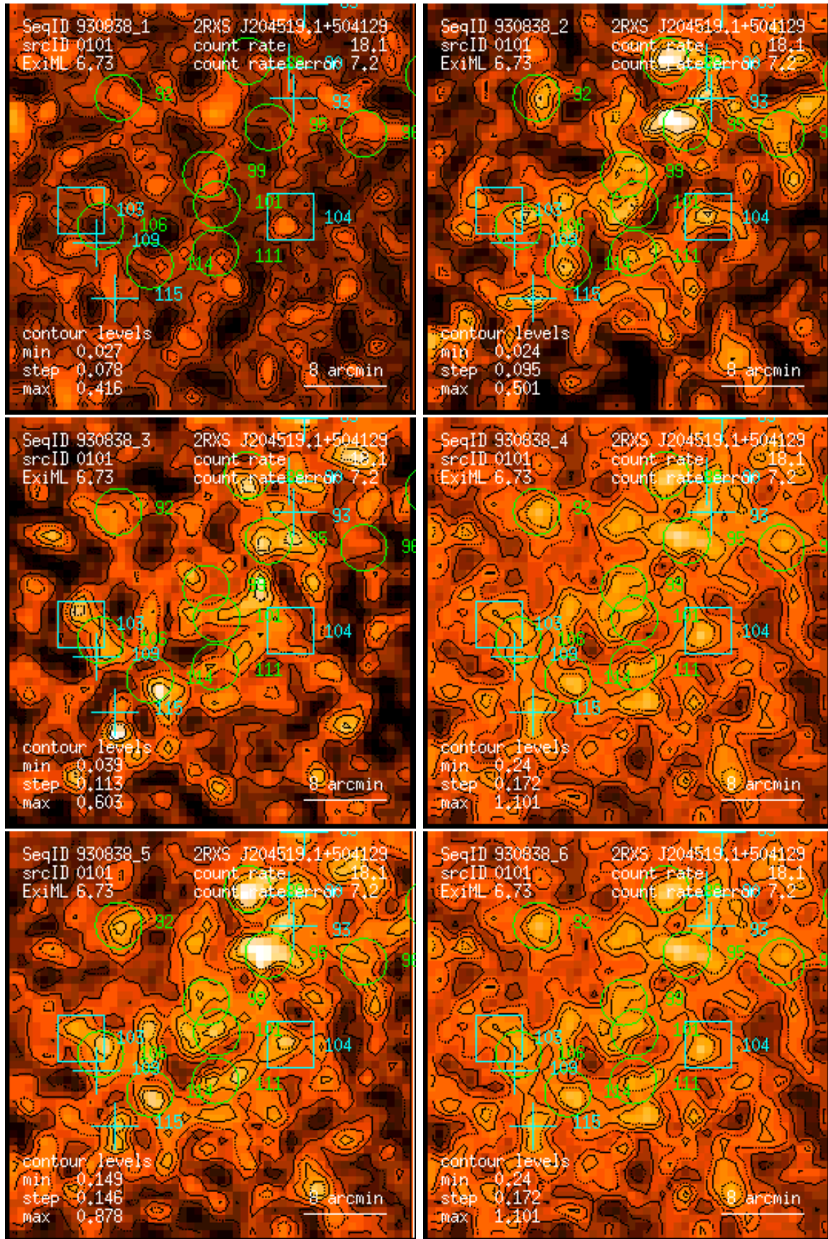
Figure 101: RASS 930838: detection 0101: band rate images, Gaussian filter: (1) PSPC channels 11 – 41, (2) 52 – 90, (3) 91 – 201, (4) 11 – 235, (5) 52 – 201, (6) 11 – 201. Broad band rates in counts/ks. Band rate contour levels in counts/ks/arcmin 2 .
