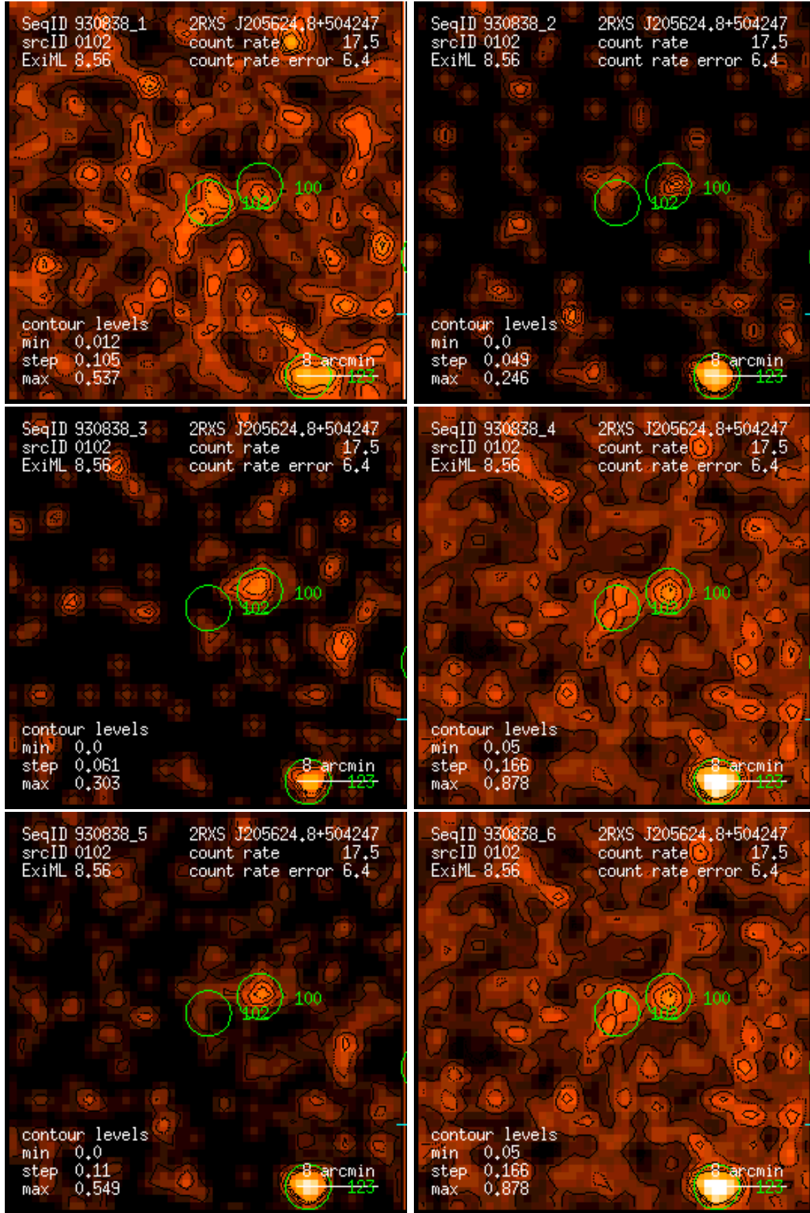
Figure 102: RASS 930838: detection 0102: band rate images, Gaussian filter: (1) PSPC channels 11 – 41, (2) 52 – 90, (3) 91 – 201, (4) 11 – 235, (5) 52 – 201, (6) 11 – 201. Broad band rates in counts/ks. Band rate contour levels in counts/ks/arcmin 2 .
