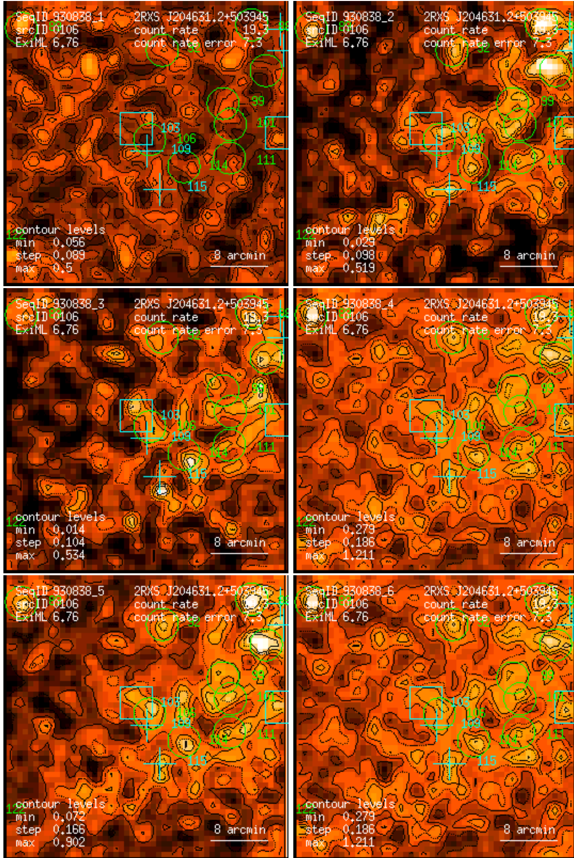
Figure 106: RASS 930838: detection 0106: band rate images, Gaussian filter: (1) PSPC channels 11 – 41, (2) 52 – 90, (3) 91 – 201, (4) 11 – 235, (5) 52 – 201, (6) 11 – 201. Broad band rates in counts/ks. Band rate contour levels in counts/ks/arcmin 2 .
