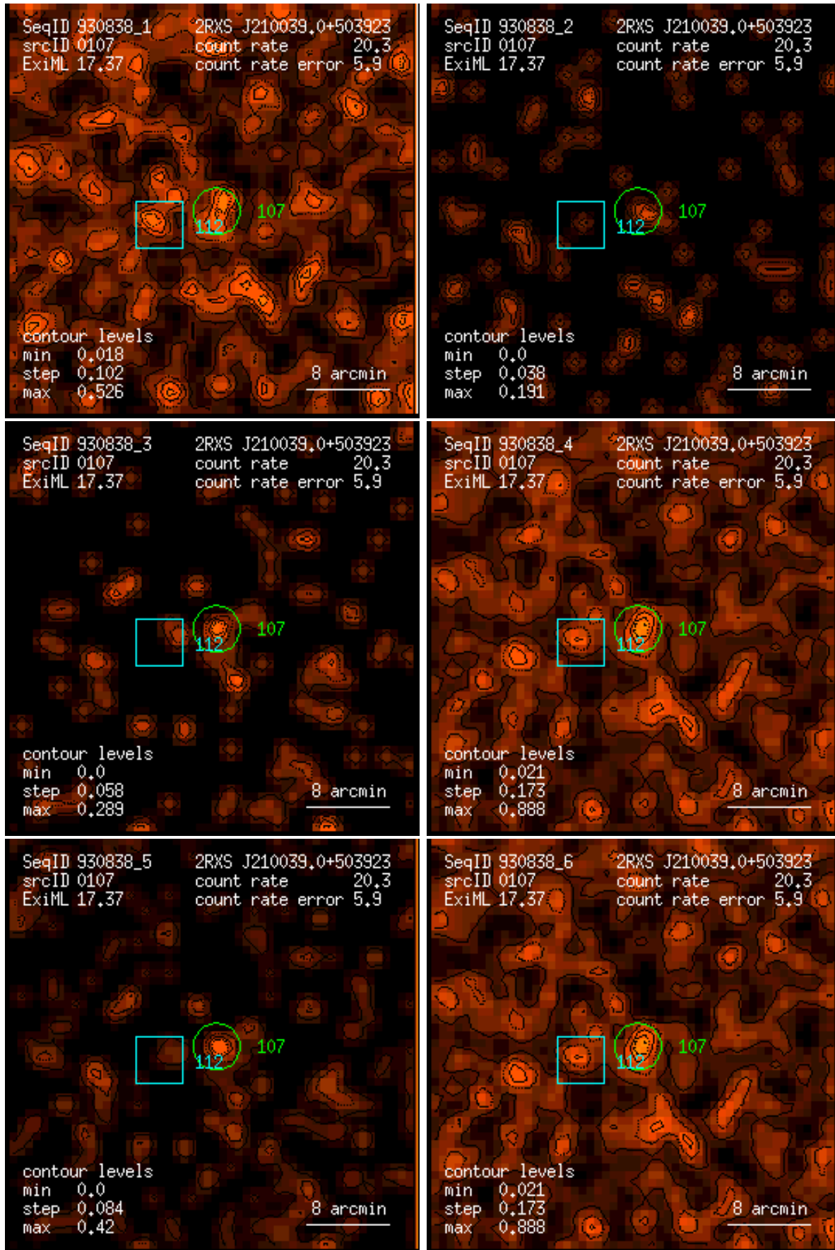
Figure 107: RASS 930838: detection 0107: band rate images, Gaussian filter: (1) PSPC channels 11 – 41, (2) 52 – 90, (3) 91 – 201, (4) 11 – 235, (5) 52 – 201, (6) 11 – 201. Broad band rates in counts/ks. Band rate contour levels in counts/ks/arcmin 2 .
