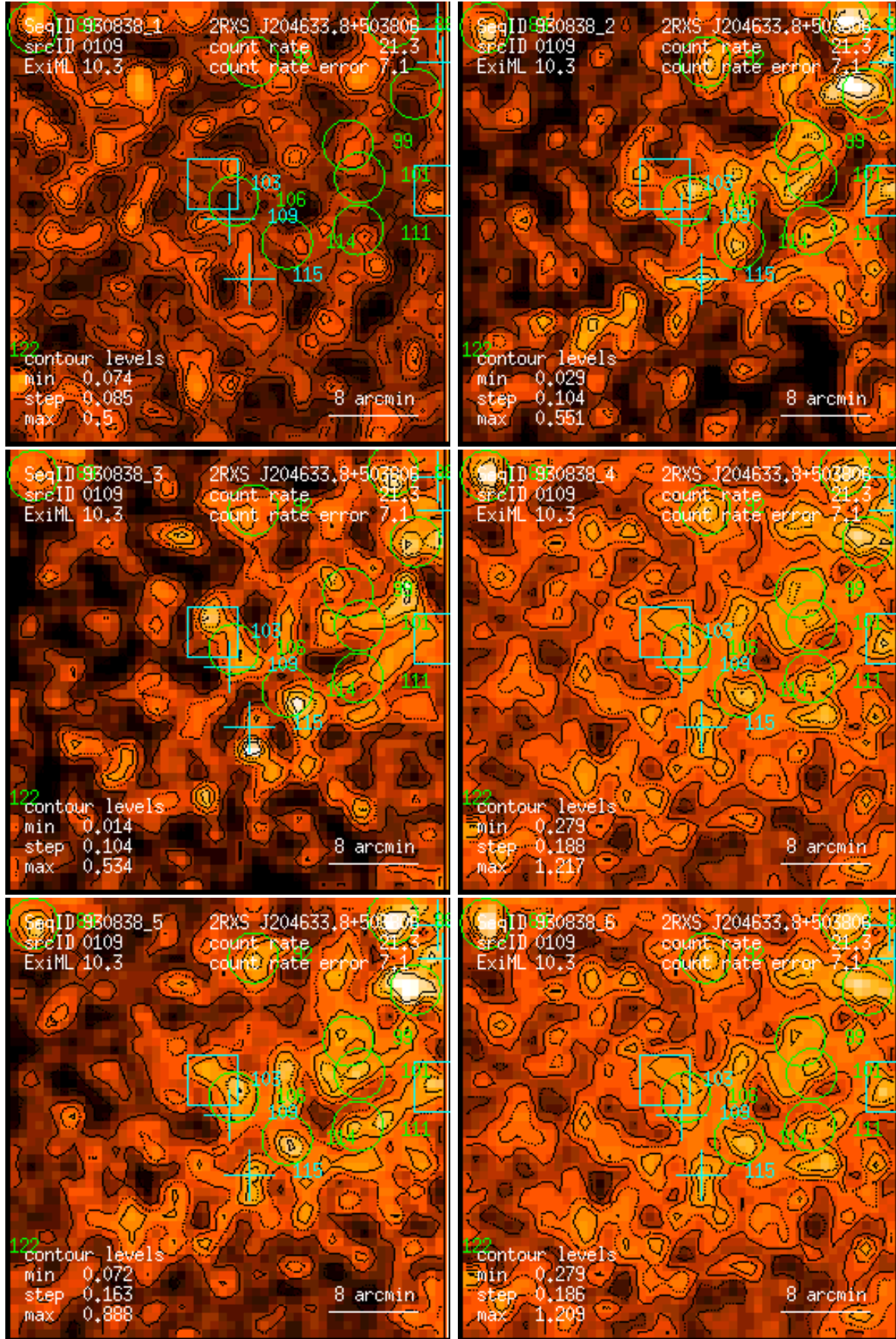
Figure 109: RASS 930838: detection 0109: band rate images, Gaussian filter: (1) PSPC channels 11 – 41, (2) 52 – 90, (3) 91 – 201, (4) 11 – 235, (5) 52 – 201, (6) 11 – 201. Broad band rates in counts/ks. Band rate contour levels in counts/ks/arcmin 2 .
