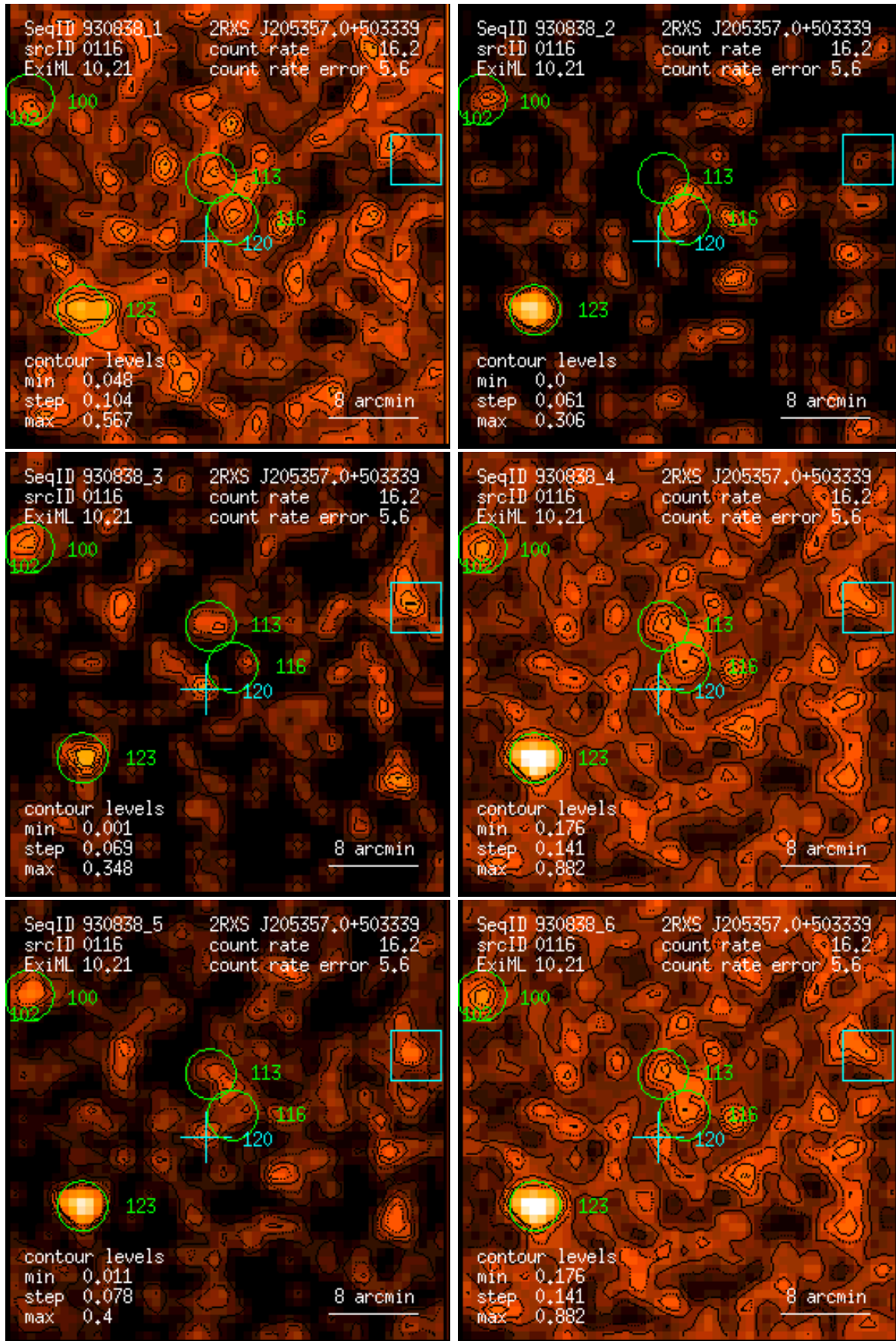
Figure 116: RASS 930838: detection 0116: band rate images, Gaussian filter: (1) PSPC channels 11 – 41, (2) 52 – 90, (3) 91 – 201, (4) 11 – 235, (5) 52 – 201, (6) 11 – 201. Broad band rates in counts/ks. Band rate contour levels in counts/ks/arcmin 2 .
