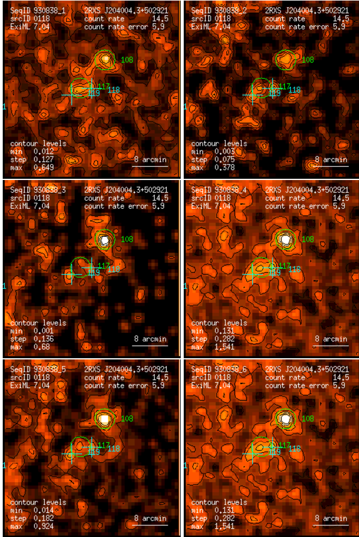
Figure 118: RASS 930838: detection 0118: band rate images, Gaussian filter: (1) PSPC channels 11 – 41, (2) 52 – 90, (3) 91 – 201, (4) 11 – 235, (5) 52 – 201, (6) 11 – 201. Broad band rates in counts/ks. Band rate contour levels in counts/ks/arcmin 2 .
