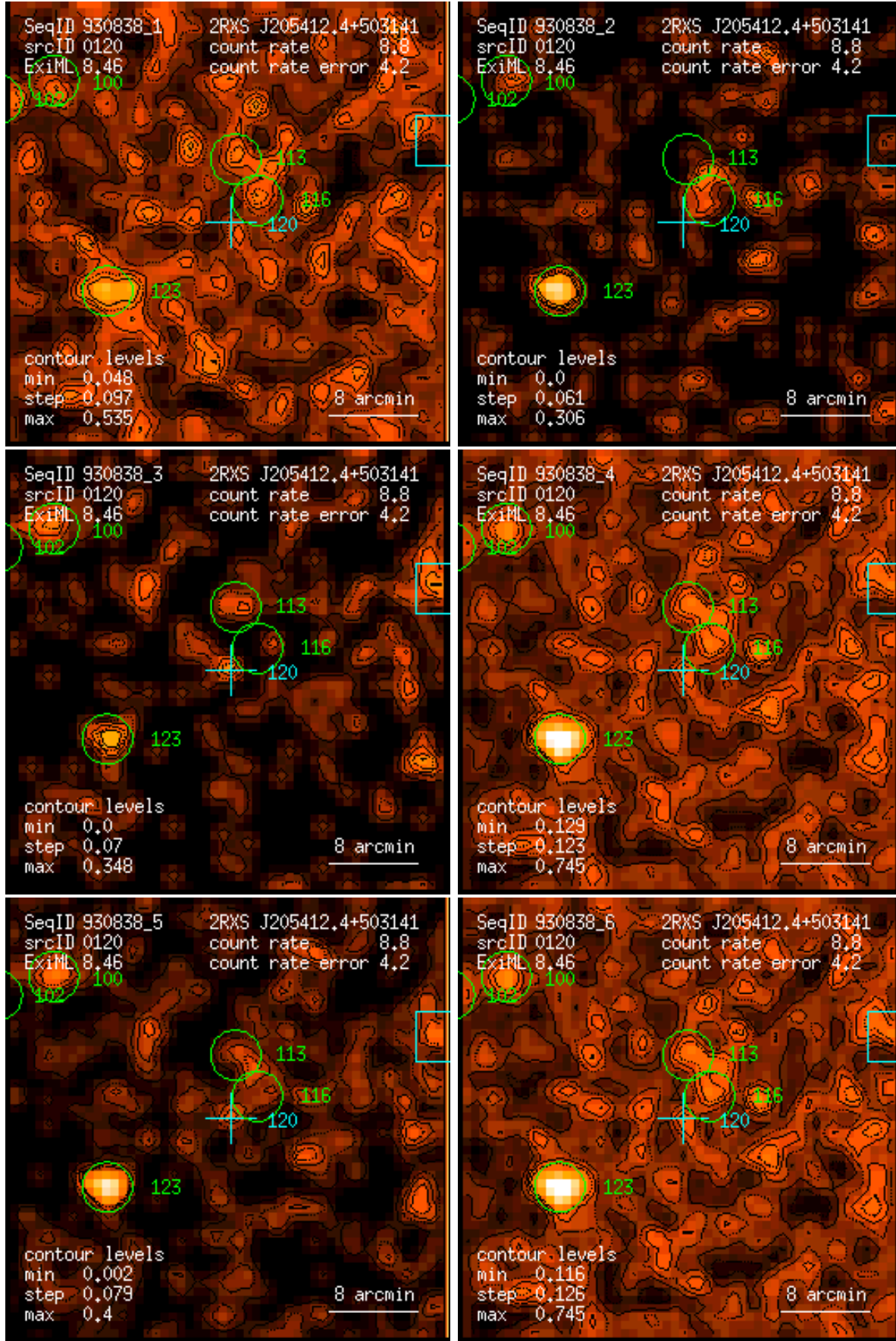
Figure 120: RASS 930838: detection 0120: band rate images, Gaussian filter: (1) PSPC channels 11 – 41, (2) 52 – 90, (3) 91 – 201, (4) 11 – 235, (5) 52 – 201, (6) 11 – 201. Broad band rates in counts/ks. Band rate contour levels in counts/ks/arcmin 2 .
