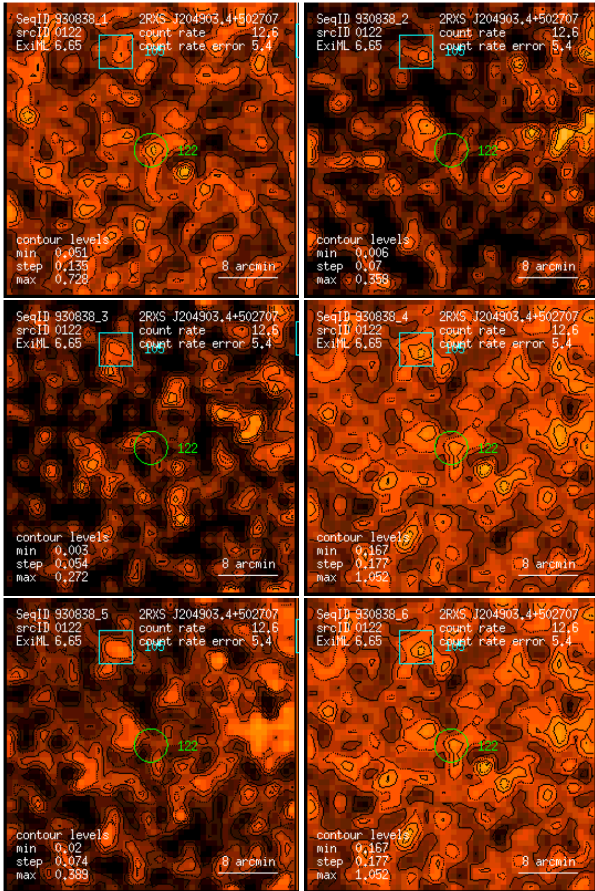
Figure 122: RASS 930838: detection 0122: band rate images, Gaussian filter: (1) PSPC channels 11 – 41, (2) 52 – 90, (3) 91 – 201, (4) 11 – 235, (5) 52 – 201, (6) 11 – 201. Broad band rates in counts/ks. Band rate contour levels in counts/ks/arcmin 2 .
