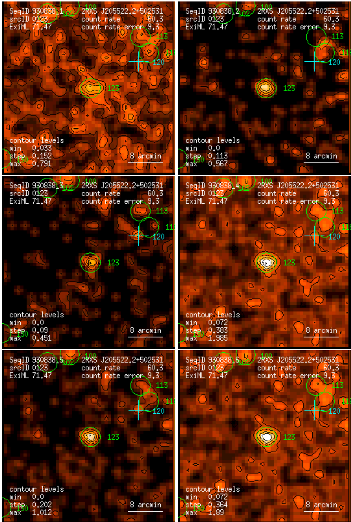
Figure 123: RASS 930838: detection 0123: band rate images, Gaussian filter: (1) PSPC channels 11 – 41, (2) 52 – 90, (3) 91 – 201, (4) 11 – 235, (5) 52 – 201, (6) 11 – 201. Broad band rates in counts/ks. Band rate contour levels in counts/ks/arcmin 2 .
