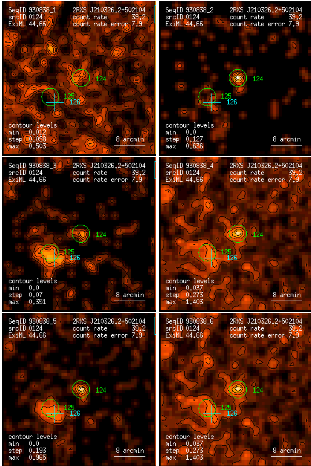
Figure 124: RASS 930838: detection 0124: band rate images, Gaussian filter: (1) PSPC channels 11 – 41, (2) 52 – 90, (3) 91 – 201, (4) 11 – 235, (5) 52 – 201, (6) 11 – 201. Broad band rates in counts/ks. Band rate contour levels in counts/ks/arcmin 2 .
