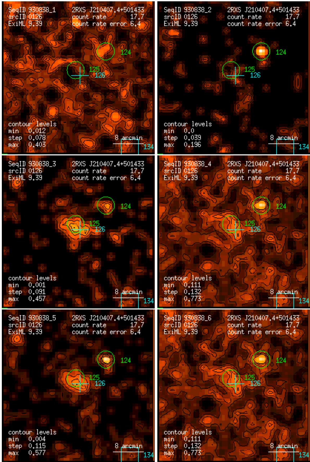
Figure 126: RASS 930838: detection 0126: band rate images, Gaussian filter: (1) PSPC channels 11 – 41, (2) 52 – 90, (3) 91 – 201, (4) 11 – 235, (5) 52 – 201, (6) 11 – 201. Broad band rates in counts/ks. Band rate contour levels in counts/ks/arcmin 2 .
