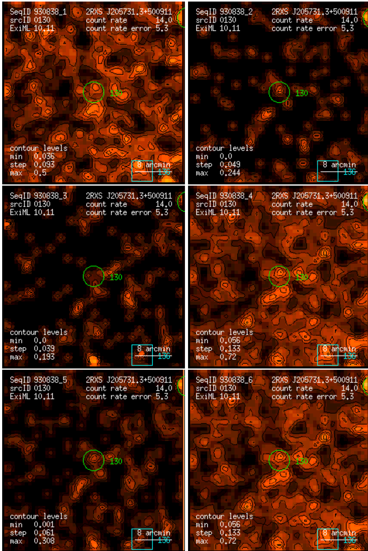
Figure 130: RASS 930838: detection 0130: band rate images, Gaussian filter: (1) PSPC channels 11 – 41, (2) 52 – 90, (3) 91 – 201, (4) 11 – 235, (5) 52 – 201, (6) 11 – 201. Broad band rates in counts/ks. Band rate contour levels in counts/ks/arcmin 2 .
