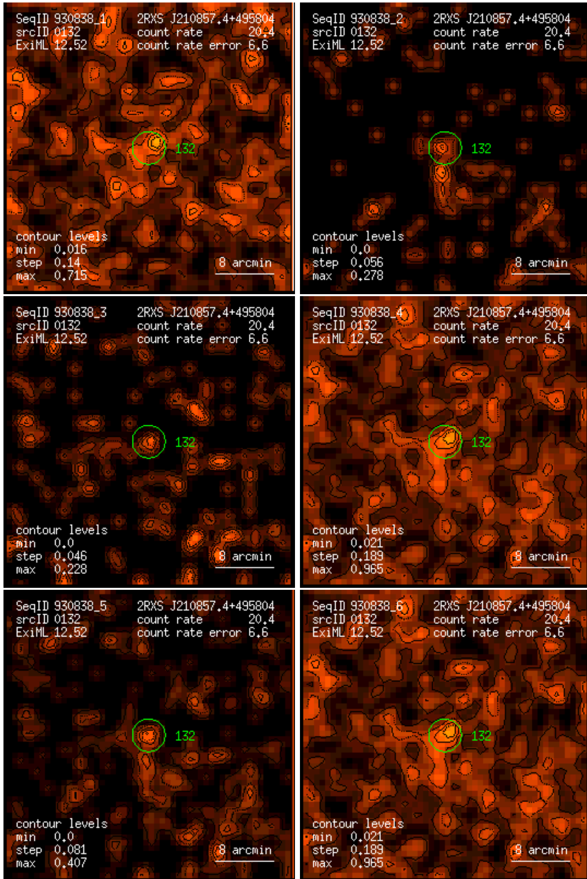
Figure 132: RASS 930838: detection 0132: band rate images, Gaussian filter: (1) PSPC channels 11 – 41, (2) 52 – 90, (3) 91 – 201, (4) 11 – 235, (5) 52 – 201, (6) 11 – 201. Broad band rates in counts/ks. Band rate contour levels in counts/ks/arcmin 2 .
