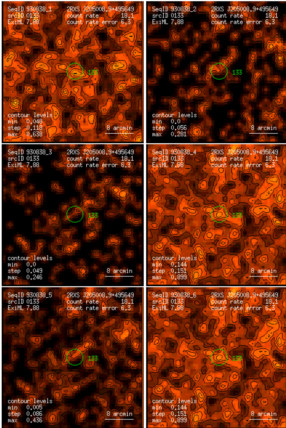
Figure 133: RASS 930838: detection 0133: band rate images, Gaussian filter: (1) PSPC channels 11 – 41, (2) 52 – 90, (3) 91 – 201, (4) 11 – 235, (5) 52 – 201, (6) 11 – 201. Broad band rates in counts/ks. Band rate contour levels in counts/ks/arcmin 2 .
