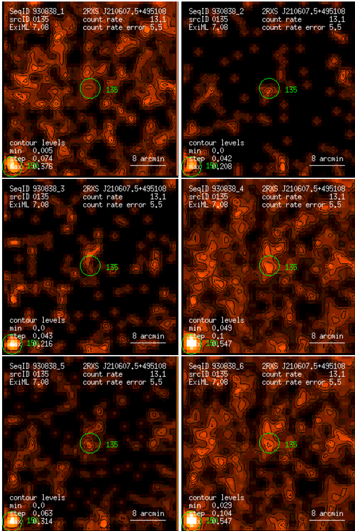
Figure 135: RASS 930838: detection 0135: band rate images, Gaussian filter: (1) PSPC channels 11 – 41, (2) 52 – 90, (3) 91 – 201, (4) 11 – 235, (5) 52 – 201, (6) 11 – 201. Broad band rates in counts/ks. Band rate contour levels in counts/ks/arcmin 2 .
