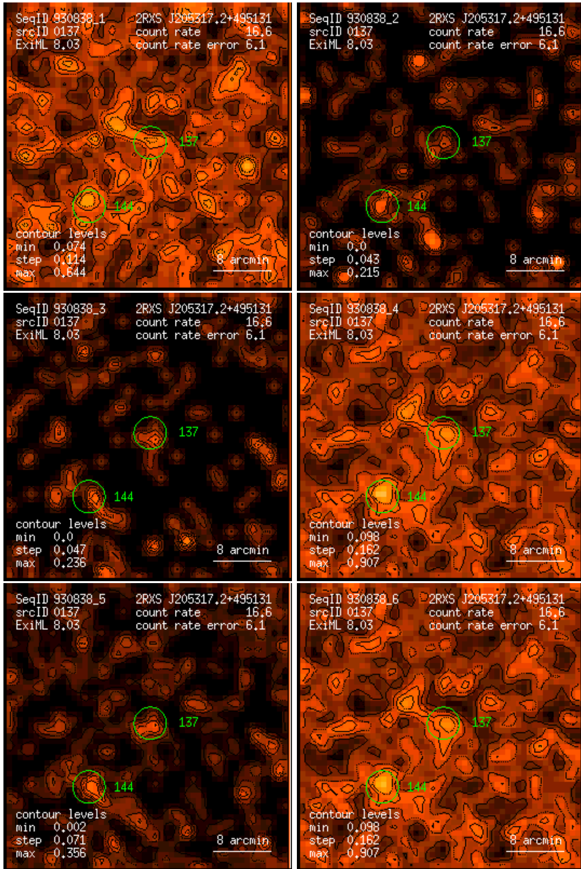
Figure 137: RASS 930838: detection 0137: band rate images, Gaussian filter: (1) PSPC channels 11 – 41, (2) 52 – 90, (3) 91 – 201, (4) 11 – 235, (5) 52 – 201, (6) 11 – 201. Broad band rates in counts/ks. Band rate contour levels in counts/ks/arcmin 2 .
