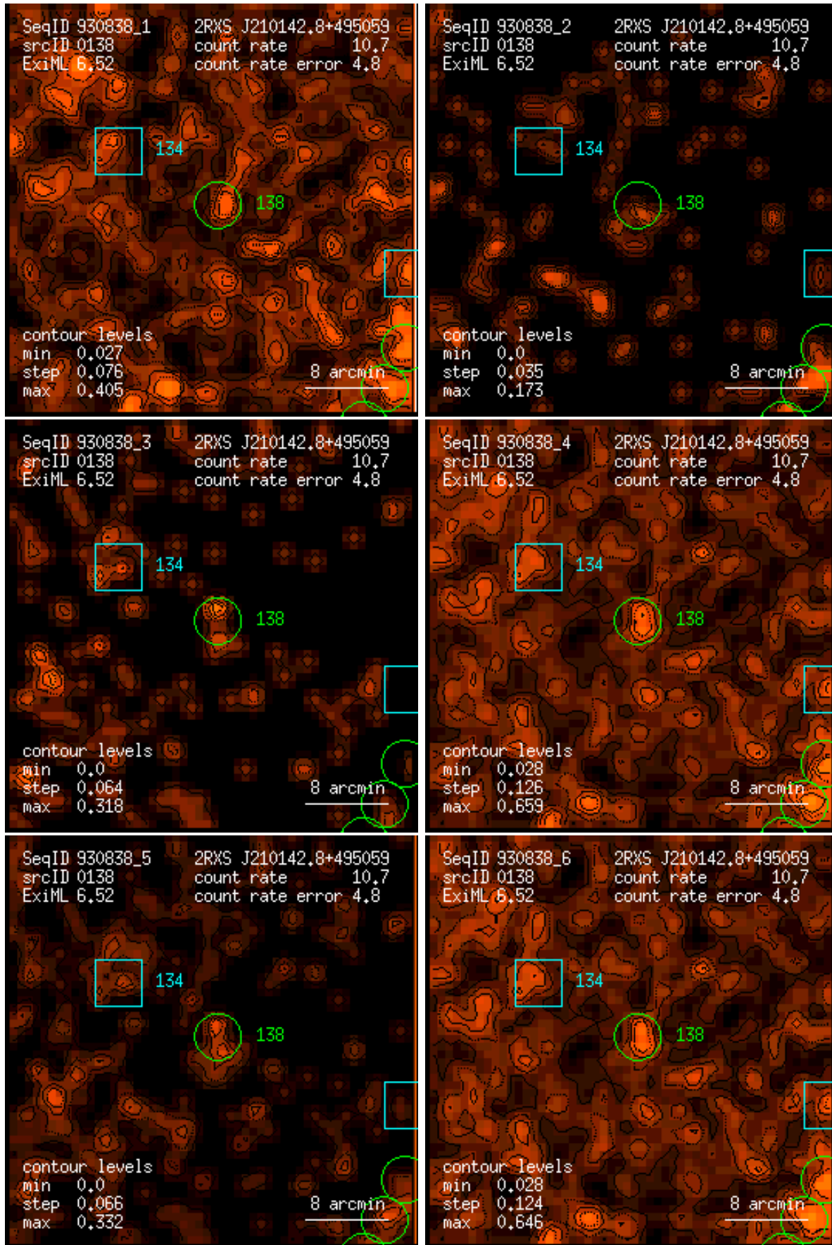
Figure 138: RASS 930838: detection 0138: band rate images, Gaussian filter: (1) PSPC channels 11 – 41, (2) 52 – 90, (3) 91 – 201, (4) 11 – 235, (5) 52 – 201, (6) 11 – 201. Broad band rates in counts/ks. Band rate contour levels in counts/ks/arcmin 2 .
