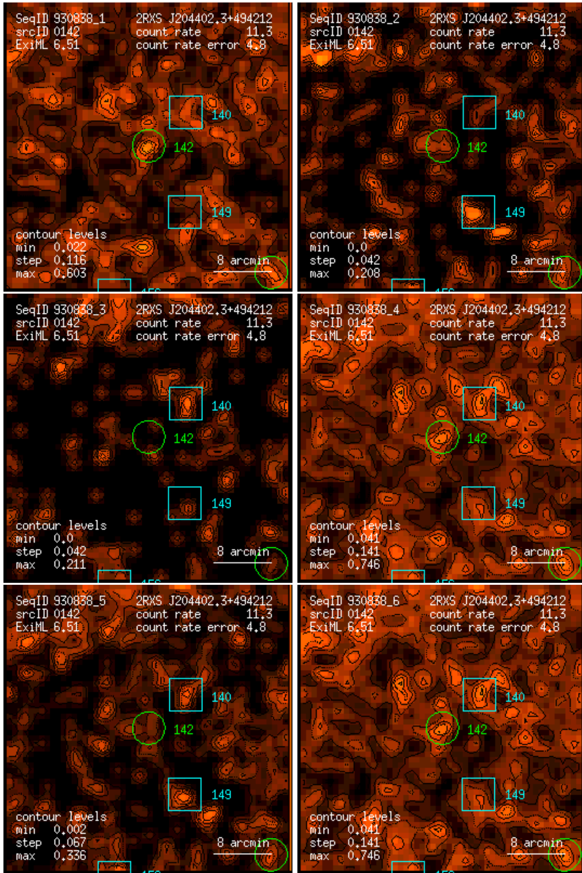
Figure 142: RASS 930838: detection 0142: band rate images, Gaussian filter: (1) PSPC channels 11 – 41, (2) 52 – 90, (3) 91 – 201, (4) 11 – 235, (5) 52 – 201, (6) 11 – 201. Broad band rates in counts/ks. Band rate contour levels in counts/ks/arcmin 2 .
