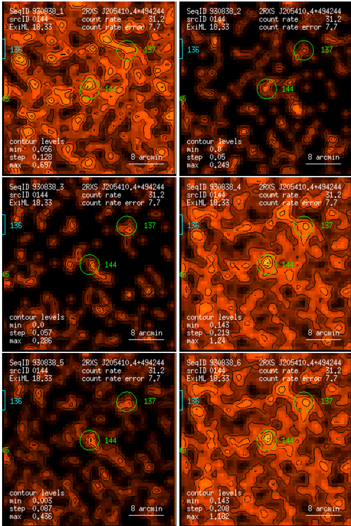
Figure 144: RASS 930838: detection 0144: band rate images, Gaussian filter: (1) PSPC channels 11 – 41, (2) 52 – 90, (3) 91 – 201, (4) 11 – 235, (5) 52 – 201, (6) 11 – 201. Broad band rates in counts/ks. Band rate contour levels in counts/ks/arcmin 2 .
